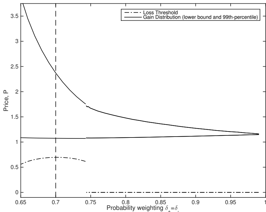
Figure 5: Summary statistics for the optimal quantile function in the model with Tversky and Kahneman value and weighting functions. The figure shows the location of the single loss threshold and the location of the mass on gains together with the upper 99th percentile of the distribution, each as a function of the probability weighting parameter \delta_+ = \delta_- = \delta . The vertical dashed line indicates the base parameter value of \delta_{\pm} = 0.7 . Base parameters used are \alpha_+ = 0.5 , \alpha_- = 0.9 , loss aversion parameter k = 1.25 , \beta = 0.9 , reference level R = 1 and P_0 = 1 . Note that a loss threshold of zero in the figures represents the situation where the investor never voluntarily realizes losses.
