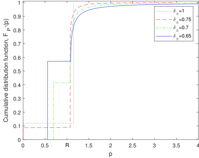
Figure 2: Cumulative distribution function (CDF) plots for the optimal prospect in the model with Tversky and Kahneman value and weighting functions, for different values of probability weighting parameter \delta = \delta_+ = \delta_- . For weak probability weighting ( \delta > 0.74 ) the mass on losses is at zero, but for sufficiently strong probability weighting ( \delta < 0.74 ) the mass on losses is at a strictly positive level. We set the reference level R = 1 and initial asset price P_0 = 1 . Other base parameters are \alpha_+ = 0.5 , \alpha_- = 0.9 , loss aversion parameter k = 1.25 , \beta = 1 - 2\kappa/\sigma^2 = 0.9 (where \kappa is the asset's expected return and \sigma the volatility of asset returns). The base case TK model and parameters are described in Section 5.
