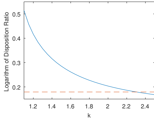
(b) Loss aversion k varying
