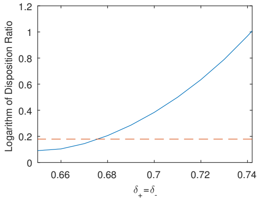
(a) Probability weighting \delta_+ = \delta_- varying
