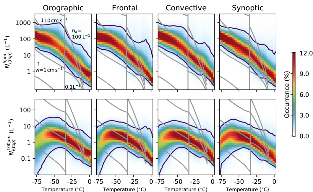
Figure 2. The conditional N_{i(\text{top})} ( L^{-1} ) for 5^{\circ}\text{C} temperature bins for each of the main cloud regimes (orographic, frontal, convective and synoptic) from Gryspeerd et al. (2018a, O2, F, C and S). The top row shows the N_{i(\text{top})} for particles greater than 5\mu\text{m} ( N_{i(\text{top})}^{5\mu\text{m}} ) and the bottom row shows the N_{i(\text{top})} for particles greater than 100\mu\text{m} ( N_{i(\text{top})}^{100\mu\text{m}} ). The columns are normalized so that they sum to 100%. The vertical line is drawn at -35^{\circ}\text{C} – approximately the homogeneous nucleation threshold temperature. At temperatures warmer than -35^{\circ}\text{C} , the grid lines show the INP numbers predicted by the DeMott et al. (2010) parameterization for 0.1, 1, 10 and 100 L^{-1} aerosols > 0.5\mu\text{m} . The grid lines at temperatures below -35^{\circ}\text{C} are the N_i values following Koop et al. (2000) for 1, 10 and 100 \text{ cm s}^{-1} updraft speeds for a mean pressure and an aerosol particle number of 300 \text{ cm}^{-3} , following Krämer et al. (2009). The regime names and definitions are given in Table 1 of Gryspeerd et al. (2017). Note the log scale for N_{i(\text{top})} .
