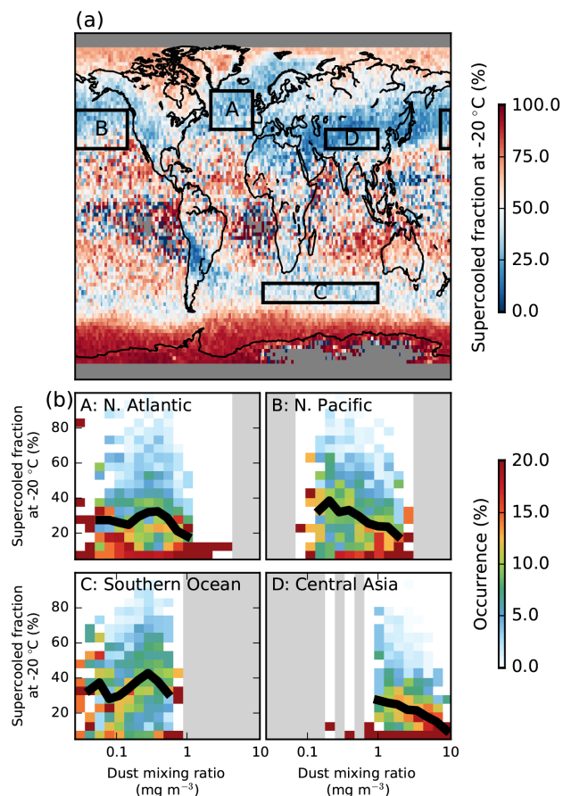
Figure 7. (a) The DARDAR supercooled fraction at -20^{\circ}\text{C} , defined as the fraction of the DARDAR cloud top phase retrievals between -17.5 and -22.5^{\circ}\text{C} from 2006 and 2013 that are classed as liquid. (b) The conditional probability of observing a daily mean supercooled fraction, given a specified MACC dust mixing ratio for the regions specified in (a). The black line shows the mean supercooled fraction for each aerosol bin.
