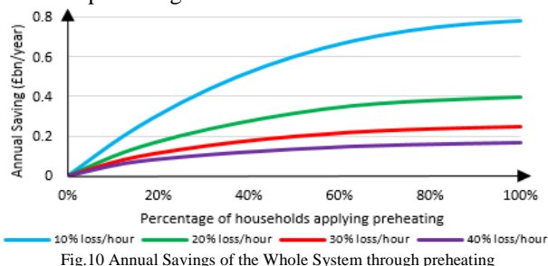
Fig.10 Annual Savings of the Whole System through preheating
