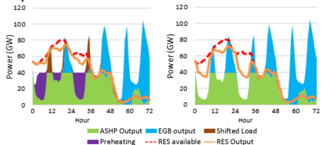
Fig.9 Operating patterns of hybrid HP-Bs with (a) and without (b) preheating
