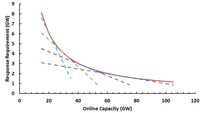
Fig.2 Piecewise linear function of frequency requirement of the system
