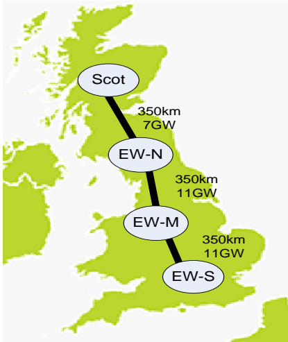
Fig.4: Schematic topology and the existing capacity of the GB transmission links between the key regions
