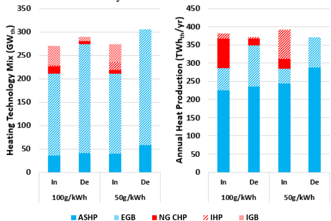
Fig.8 (a) Heating technology mix and (b) annual heat production of integrated and decoupled cases under different carbon scenarios
