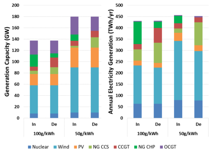
Fig.6: (a) Generation mix and (b) annual electricity generation of integrated and decoupled cases under different carbon scenarios
