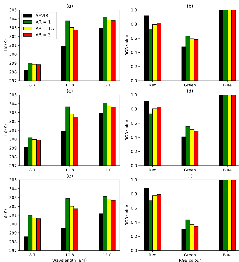
Figure 11. Mean brightness temperatures (left column) and RGB colours (right column) across the domain for the three ranges of surface emissivity values, for the SEVIRI measurements and retrievals and tested for the VO73 dust simulations with the three (horizontally aligned) aspect ratios of 1, 1.7, and 2, for the June and July of 2011–2013. Only points with AODs between 2 and 3 are included. Using emissivity at 8.7 \mu\text{m} , the panels are: (a, b) emissivity from 0.7–0.8; (c, d) 0.8–0.9; (e, f) 0.9–1.0.
