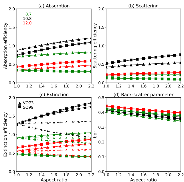
Figure 7. Plots of the derived (a) absorption, (b) scattering, (c) extinction efficiencies, and (d) back-scatter parameters (bpr) for the VO73 and SO99 dust types. These are presented here as a function of particle aspect ratio, for COSMO-MUSCAT dust size bin 3 ( r_{\text{eff}} = 1.51 \mu\text{m} ) for the three MSG-3 SEVIRI channels at 8.7, 10.8, and 12.0 \mu\text{m} . The solid lines are for horizontally aligned particles, the dashed lines for randomly oriented particles (open symbols) and for vertically oriented particles (filled symbols). For clarity, the randomly and vertically oriented cases are only included in the extinctions for VO73 dust.
