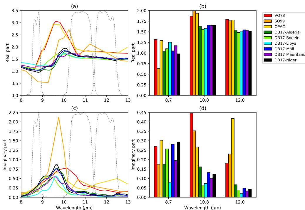
Figure 4. Plots of the real ( a, b ) and imaginary ( c, d ) parts of the dust refractive index, for nine of the dust databases considered in this study. For the left panels ( a, c ) the refractive indices are shown as a function of wavelength, as specified by their databases; the grey dashed lines indicate the relevant MSG-3 SEVIRI filter functions, normalized to the scale of the y-axis. For the right panels ( b, d ) the refractive indices have been convolved across these MSG-3 SEVIRI filter functions.
