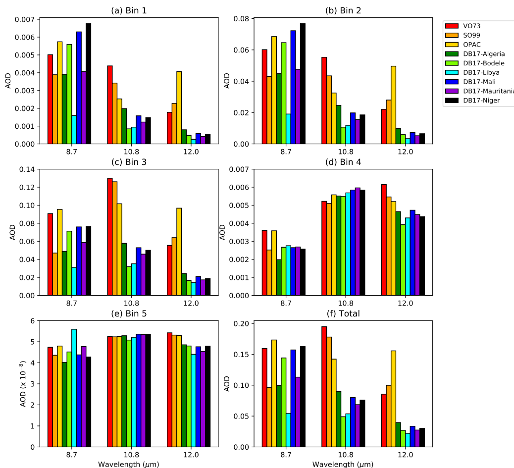
Figure 5. Plots of atmospheric column-integrated IR AODs for the five size bins and their total, over the BBM site in southern Algeria (21.38° N, 0.92° E), averaged for 09:00, 12:00, and 15:00 UTC for June and July 2013, for MSG-3, and for each set of IR refractive indices considered in this study. Note that each panel has a different y-axis scale, and note also that each panel is multiplied by one temporally averaged value of the column-integrated number density, so the pattern of AOD within each panel is identical to the pattern of the extinction cross-section for that panel (i.e. for any panel the value of the correlation of the extinction cross-section and the AOD is 1). The particles are spherical.
