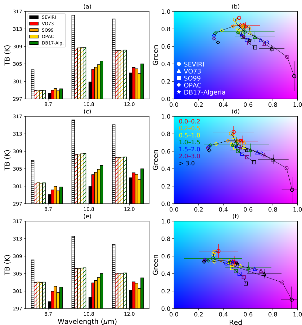
Figure 10. Mean brightness temperatures and colours across the domain for three ranges of surface emissivity values, for the SEVIRI measurements and retrievals and four of the dust simulations, for the June and July of 2011–2013. Using emissivity at 8.7\ \mu\text{m} , the panels are: (a, b) emissivity from 0.7 to 0.8; (c, d) 0.8–0.9; (e, f) 0.9–1.0. The simulated dust is spherical. Per panel of brightness temperatures (left column), within each individual wavelength set there are two groups of bars: the striped bars on the left are points with AODs between 0 and 0.2 (i.e. the most pristine-sky case); the bold bars on the right are points with AODs between 2 and 3. The mean colours (right column) are plotted within specified AOD ranges denoted by the coloured symbols: red is 0–0.2; orange is 0.2–0.5; yellow is 0.5–1; green is 1–1.5; blue is 1.5–2; purple is 2–3; black is > 3 . This colour coding is also marked in panel (d). The blue beam is held fixed at 1. Error bars denoting the standard deviations of the mean values are only included, for clarity, for three of the SEVIRI and the VO73 points.
