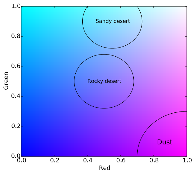
Figure 2. RGB colours as a function of red and green beams, with the blue beam fixed to a value 1. Approximate ranges of characteristic daytime colours for dust and two surface types are overlaid.
