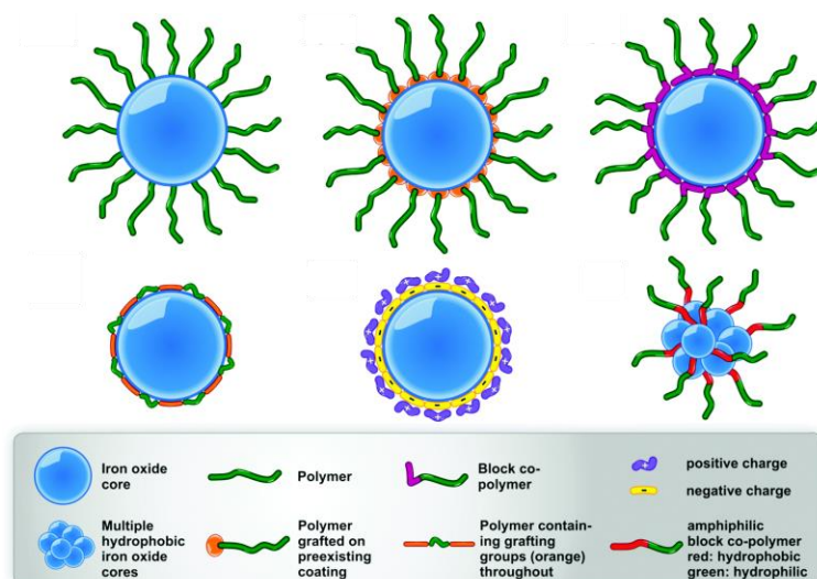
Figure 32. Schematic illustration of various polymer-iron oxide stabilization methods.
