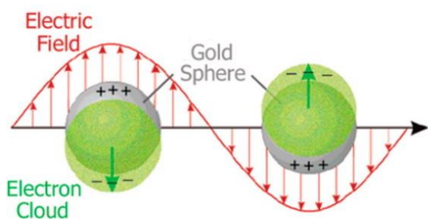
Figure 31. Schematic illustration of the oscillation of free electrons in a gold nanosphere. It is this oscillation in the presence of light that generates the localized surface plasmon resonance (LSPR). Reproduced with permission. [386] Copyright 2015, American Chemical Society.
