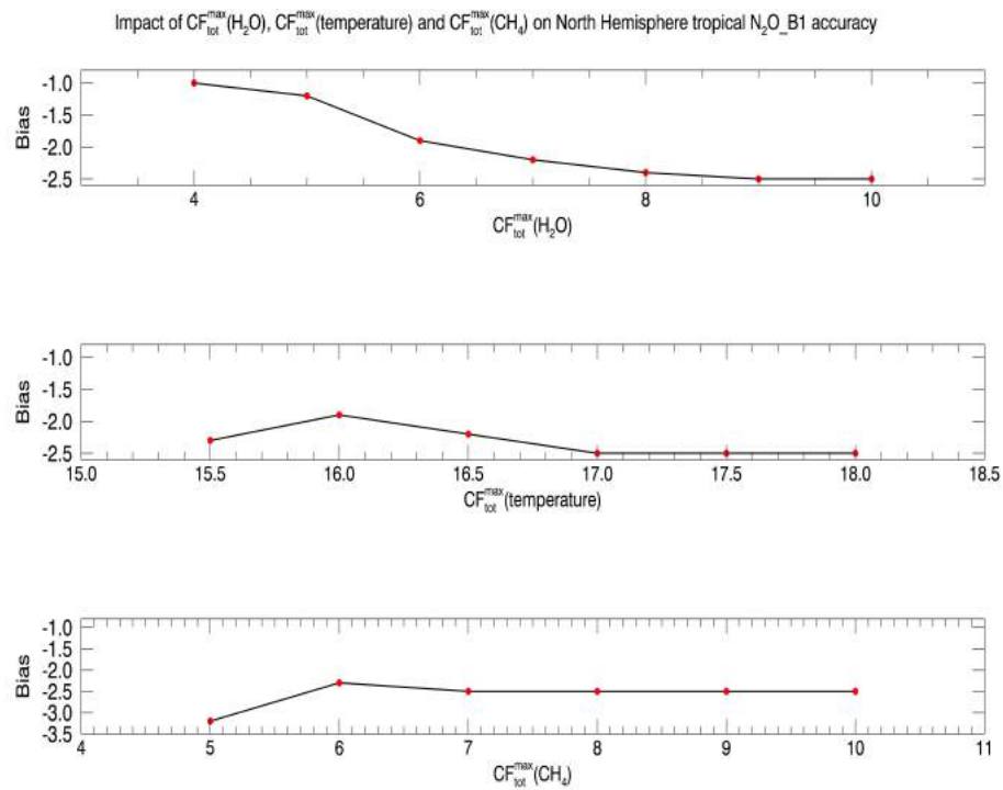
Figure 10. Mean bias corresponding to N_2O _B1-HIPPO collocated pixels in the northern hemisphere tropical regions ( 0-30^\circ N ) for different values of CF_{tot}^{max} ( H_2O ) (top), CF_{tot}^{max} (temperature) (middle) and CF_{tot}^{max} ( CH_4 ) (bottom) .
