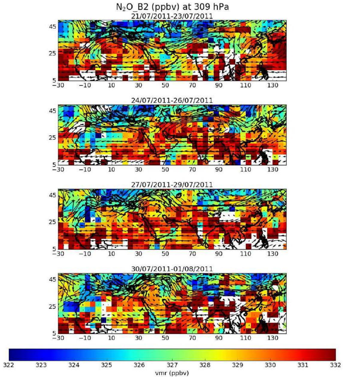
Figure 13. N_2O\_B2 at 309 hPa and horizontal winds from ERA-Interim reanalysis at 300 hPa averaged over the periods (from top to bottom) 21-23 July, 24-26 July, 27-29 July and 30 July-01 August 2011.
