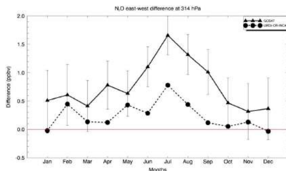
Figure 6. Seasonal variation of the east-west difference of N_2O (ppbv) measured by GOSAT TANSO-FTS (solid line) and calculated by LMDz-OR-INCA (dashed line) at 314 hPa. The error bars represent the error on the mean considering the theoretical random error of the retrieval and the number of monthly averaged pixels.
