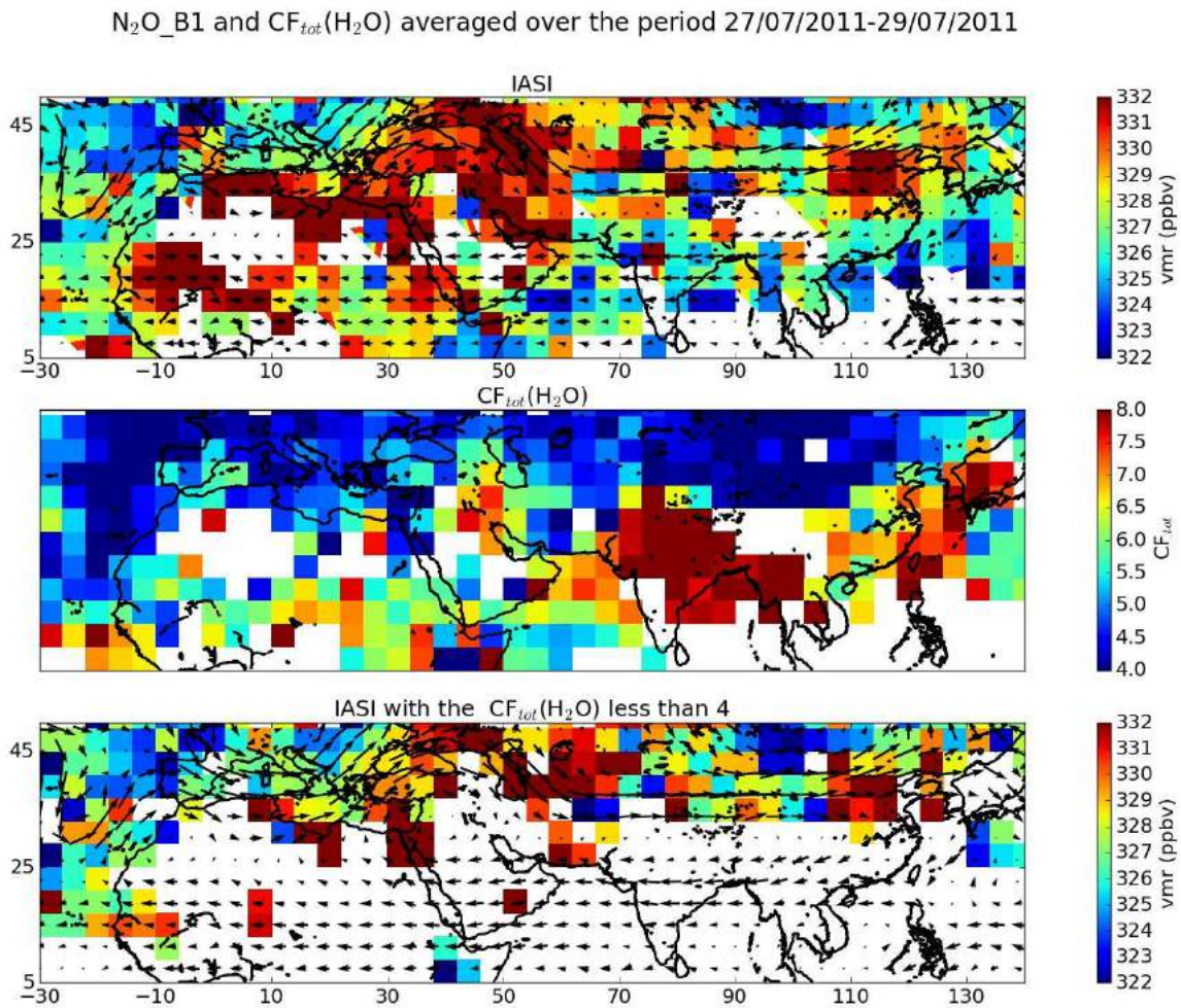
Figure 12. N 2 O_B1 (top), CF tot (H 2 O) (middle) and N 2 O_B1 filtered with CF tot max (H 2 O) equal to 4 (bottom) averaged over the period 27-29 July 2011. Horizontal winds from ERA-Interim reanalysis at 300 hPa are superimposed to N 2 O_B1.
