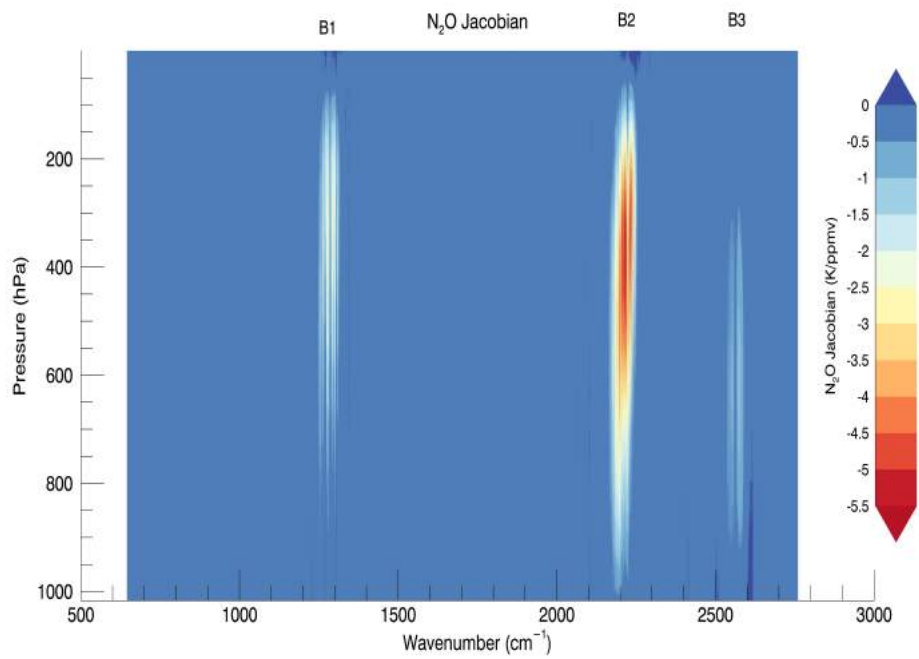
Figure 1. N 2 O Jacobian in brightness temperature calculated by RTTOV over IASI spectral range and for an atmospheric situation at 142.96°W and 11.76°N.
