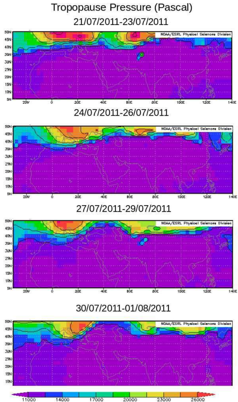
Figure 14. Tropopause pressure levels from the NCEP/NCAR 40-year reanalysis averaged over the periods (from top to bottom) 21-23 July, 24-26 July, 27-29 July and 30 July-01 August 2011.
