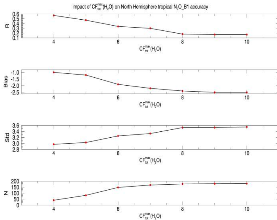
Figure 11. From top to bottom: Pearson linear correlation coefficient (R), mean bias, std error and number of IASI retrieved pixels (N) for different values of CF_{tot}^{max}(\text{H}_2\text{O}) corresponding to \text{N}_2\text{O} _B1-HIPPO collocated pixels in the northern hemisphere tropical regions ( 0\text{-}30^\circ\text{N} )
