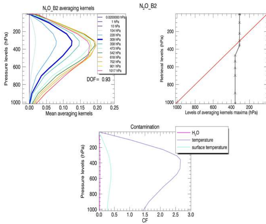
Figure 7. Same as Figure 6 for N_2O_{B2} .
