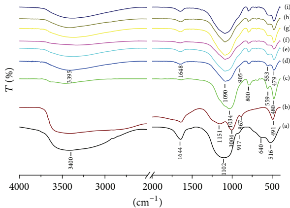
FIGURE 4: Infrared spectra of calcined Medenine clay at 700°C, phosphoric acid 85%, aluminum phosphate, and geopolymers at different molar ratios Si/P( G^x ). (a) AlPO_4 , (b) AP (85%), (c) calcined clay 700°C, (d) G^{3.5} , (e) G^{3.25} , (f) G^3 , (g) G^{2.75} , (h) G^{2.5} , and (i) G^{2.25} .
