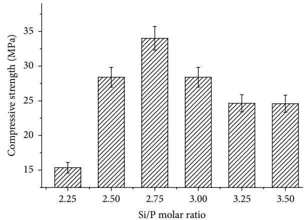
FIGURE 5: Compressive strength evolution of the phosphoric acid-based geopolymers G^x at 21 curing days for different Si/P molar ratio.
