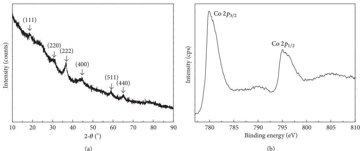
FIGURE 1: (a) X-ray diffraction pattern and (b) Co 2p XPS spectra of mesoporous \text{Co}_3\text{O}_4 nanosheets on carbon foam.
