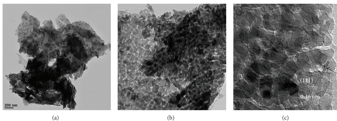
FIGURE 3: (a), (b) TEM images and (c) HRTEM image of mesoporous Co 3 O 4 nanosheets.
