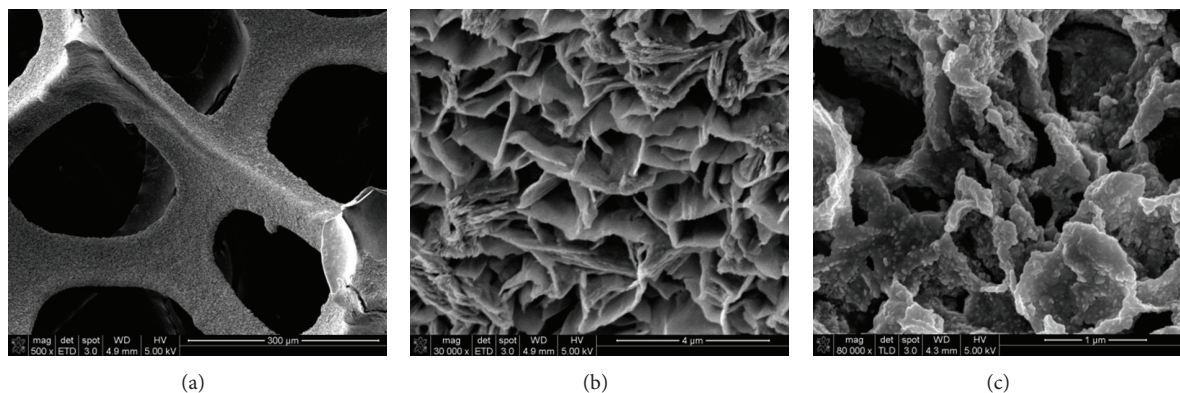
FIGURE 2: SEM images of mesoporous Co 3 O 4 nanosheets on carbon foam.
