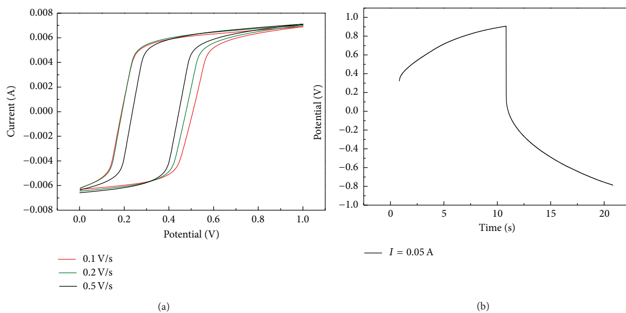
FIGURE 4: (a) Cyclic voltammetric response and (b) galvanostatic charge-discharging curve of Co 3 O 4 /carbon foam obtained in 1 M NaOH solution at different scan rates.
