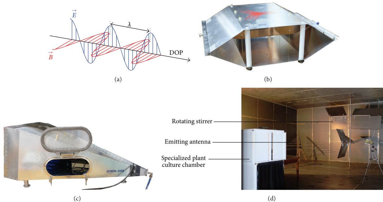
FIGURE 1: Electromagnetic wave and experimental set-up. (a) Schematic representation of an electromagnetic plane wave showing the transverse and space varying electric ( E ) and magnetic field ( B ). The wavelength ( \lambda ) is the distance between two crests. DOP: direction of propagation. (b) A TEM cell (transverse electromagnetic cell). (c) A GTEM cell (gigahertz transverse electromagnetic cell). (d) MSRC (mode stirred reverberation chamber). Note the double-sided metallic walls, the emitting antenna, the rotating stirrer, and the specialized culture chamber that stands in the “working volume” where the electromagnetic field characteristics have been extensively characterized.
