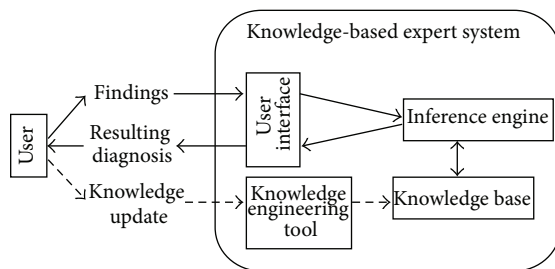
FIGURE 2: Typical structure of a knowledge-based expert system. Based on Buchanan [3], the user interface allows the nonexpert to enter the symptoms and findings [3] and presents the diagnostic output. The knowledge base provides the knowledge. Different ways of representation, such as rules, models, or cases, can be chosen. The inference engine examines the knowledge base and produces reasoning [15]. The knowledge engineering tool allows for changing or enlarging the knowledge base by adding further rules, cases, or models [7]. There may also be an explaining component, which illustrates the diagnostic process and which gives a rationale [7]. A knowledge-based expert system with an empty knowledge base is called shell. It can be used for the development of other expert systems by adding a new knowledge base [7].
