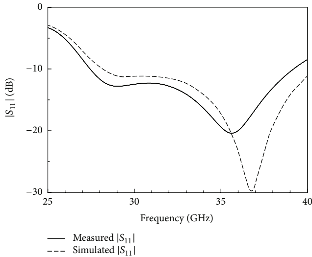
FIGURE 4: Simulated and measured return loss of the proposed antenna.
