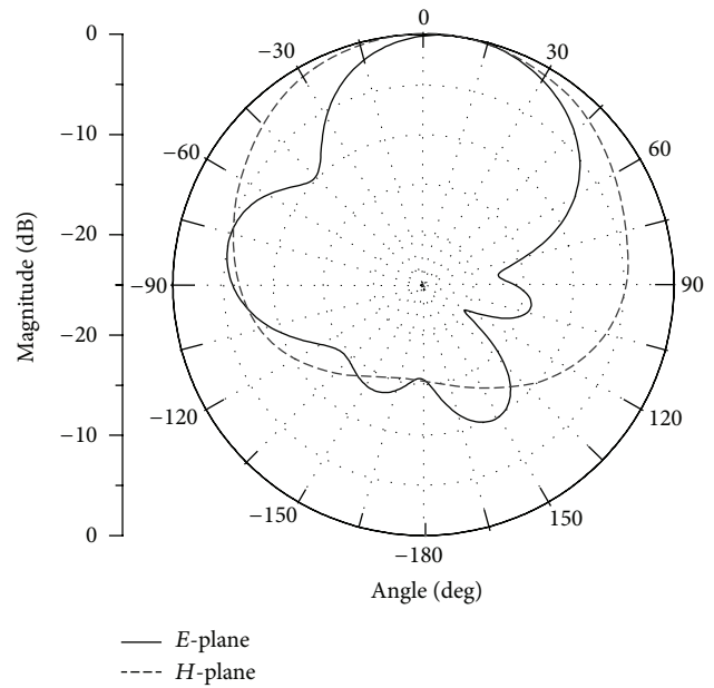
FIGURE 6: Measured far-field of the proposed PLPDA antenna at 30 GHz.
