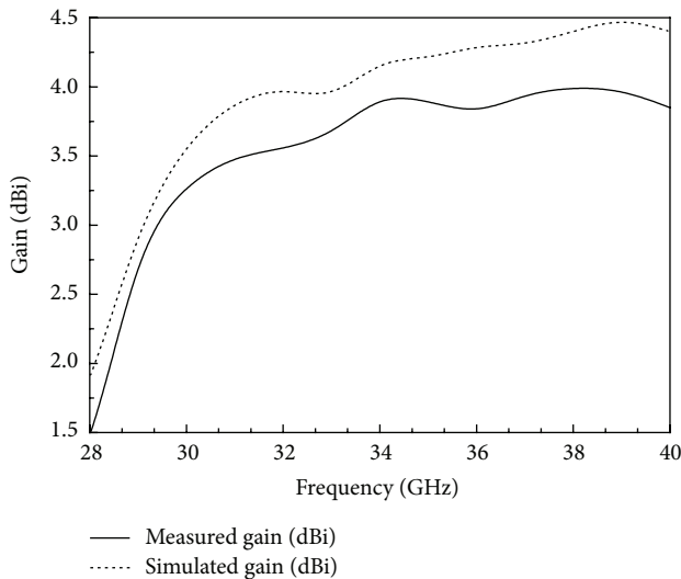
FIGURE 5: Simulated and measured gain of the proposed antenna.
