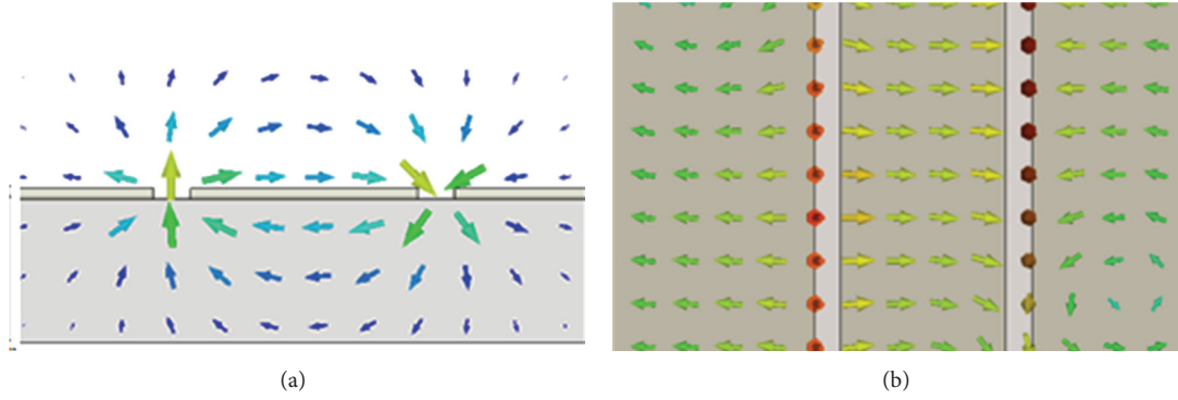
FIGURE 2: Simulated magnetic field distribution of the dominant mode in the cross view (a) and the top view (b) of the CPW.
