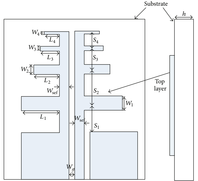
FIGURE 1: Geometry of the proposed CPW PLPDA antenna.
