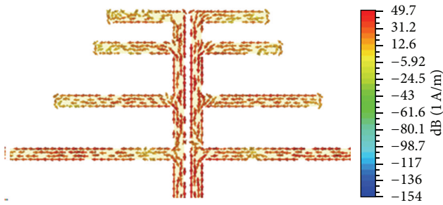
FIGURE 3: Simulated current distribution of the CPW PLPDA antenna at 35 GHz.
