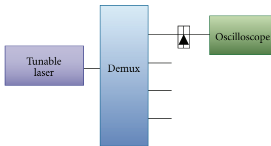
FIGURE 8: Setup for laser speed characterization.
