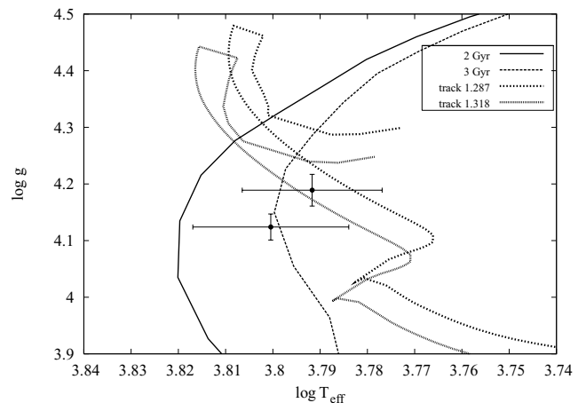
Figure 3. Evolutionary tracks for the measured masses of 1.318 and 1.287 M ⊙ and isochrones of ages of 2 and 3 Gyr generated by the YONSEI-YALE code for solar metallicity ( Z = 0.018 ) and \alpha -enhancement of zero.
