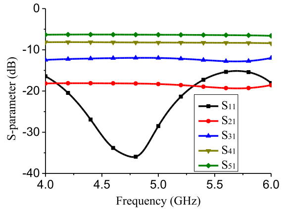
FIGURE 9. S-parameters of the simulated unequal feed network.
