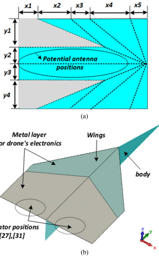
Fig. 1. Realized paper drone geometry of (a) the unfolded planar photo paper sheet and (b) perspective view of paper drone.
