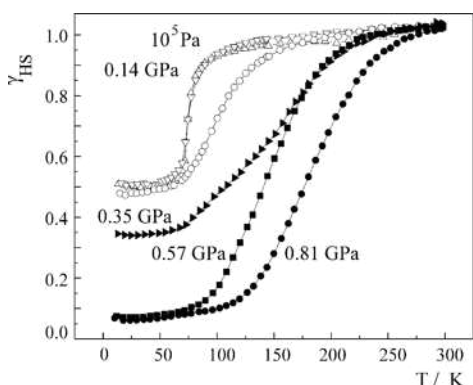
Figure 12. High spin fraction as a function of the temperature at distinct hydrostatic pressures for complex [Fe(mtz) 6 ](BF 4 ) 2 . Reprinted from [82] Copyright (2005), with permission from Elsevier
