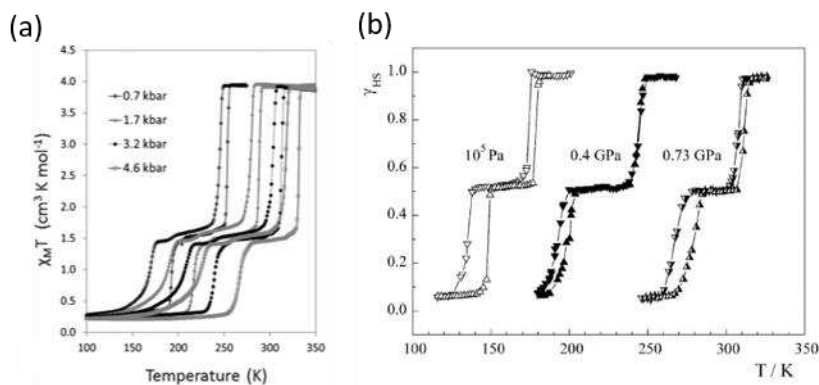
Figure 13. (a) Magnetic properties under hydrostatic pressure for [\text{Fe}(\text{babppy})(\text{NCS})_2] Reprinted with permission from [79] Copyright (2011) by the American Physical Society (b) Magnetic properties under hydrostatic pressure for [\text{Fe}(5\text{-NO}_2\text{-sal-N}(1,4,7,10))] . Reprinted from [82] Copyright (2005), with permission from Elsevier
