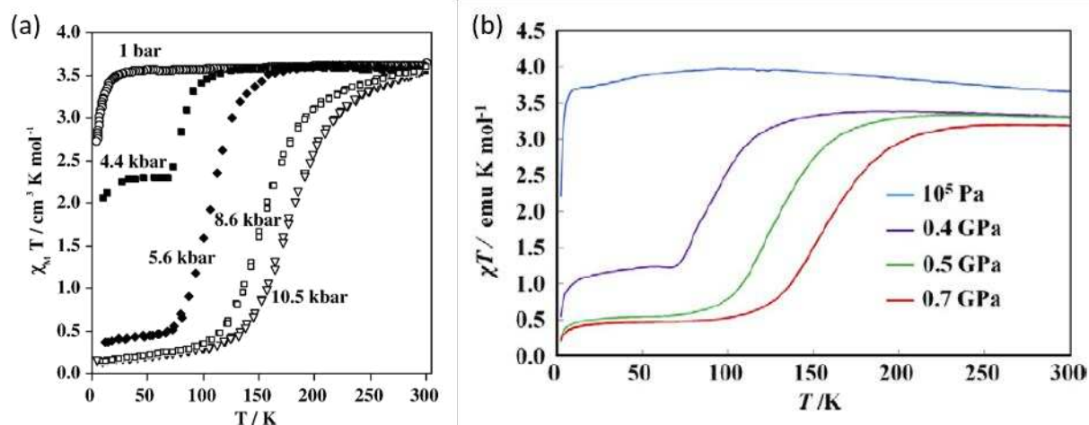
Figure 15. (a) Thermal variation of the molar magnetic susceptibility, \chi_{\text{M}}T , for [\text{Fe}(\text{abpt})_2(\text{NCS})_2] polymorph B at different hydrostatic pressures. Reprinted by permission from Springer Nature [139] (b) Thermal variation of the molar magnetic susceptibility, \chi_{\text{M}}T , for [\text{Fe}(\text{stpy})_4(\text{NCBH}_3)_2]_{\text{cis}} at different hydrostatic pressures. Reprinted from [141], Copyright (2011), with permission from Elsevier
