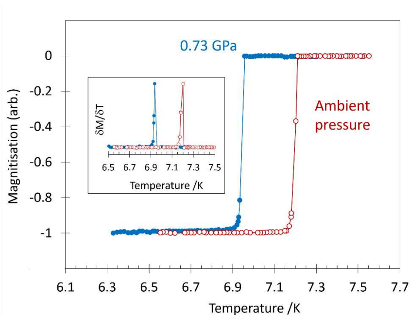
Figure 2. Illustration of the shift in temperature of the superconducting transition of Pb on the application of pressure from ambient to 0.73 GPa
