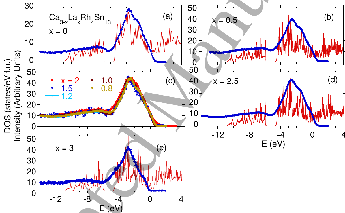
Figure A1. Valence band XPS spectra for \text{Ca}_{3-x}\text{La}_x\text{Rh}_4\text{Sn}_{13} compared with the calculated total density of states within the LSDA approximation (narrow red line) for the components x = 0, 0.5, 2.5, and 3 . The figure also shows the VB XPS spectra for intermediate components of the series [in panel (c)].
