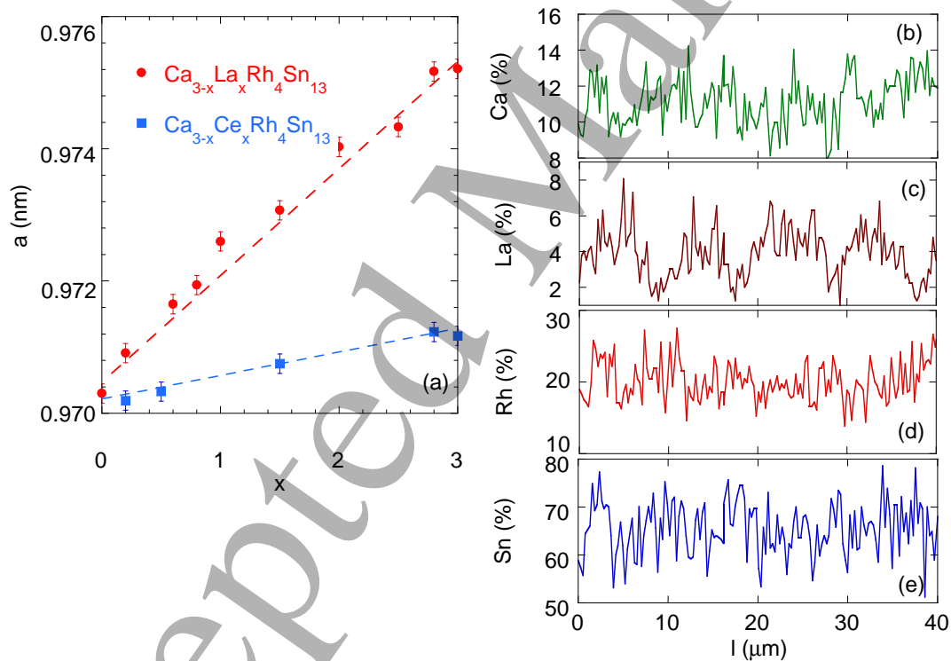
Figure 1. (a) The lattice parameter, a , plotted against La or Ce concentration, x , for the \text{Ca}_{3-x}\text{La}_x\text{Rh}_4\text{Sn}_{13} and \text{Ca}_{3-x}\text{Ce}_x\text{Rh}_4\text{Sn}_{13} series of alloys. The lattice parameters follow Vegard's law, which suggests good sample quality and stoichiometry of the components x . Panels (b), (c), (d), and (e) show variations in stoichiometry of Ca, La, Rh, and Sn, respectively over the length of the \text{Ca}_{2.2}\text{La}_{0.8}\text{Rh}_4\text{Sn}_{13} sample.
