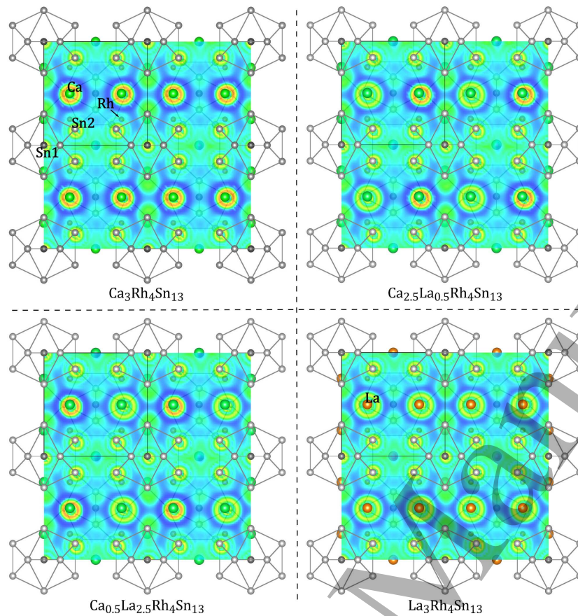
Figure A4. The ELF distribution in the plane z = 1 shown for series of compounds.
