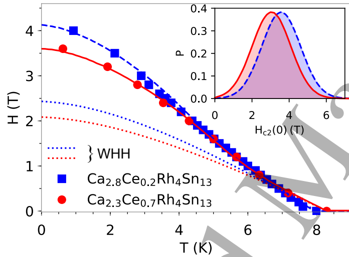
Figure 5. The upper critical field for \text{Ca}_{3-x}\text{Ce}_x\text{Rh}_4\text{Sn}_{13} for x = 0.2 and x = 0.7 fitted by results of a percolation model. The dotted lines show fits to the WHH model. The inset shows the distribution of the local H_{c2} assumed in the percolation model for x = 0.2 (dashed blue line) and x = 0.7 (solid red line).
