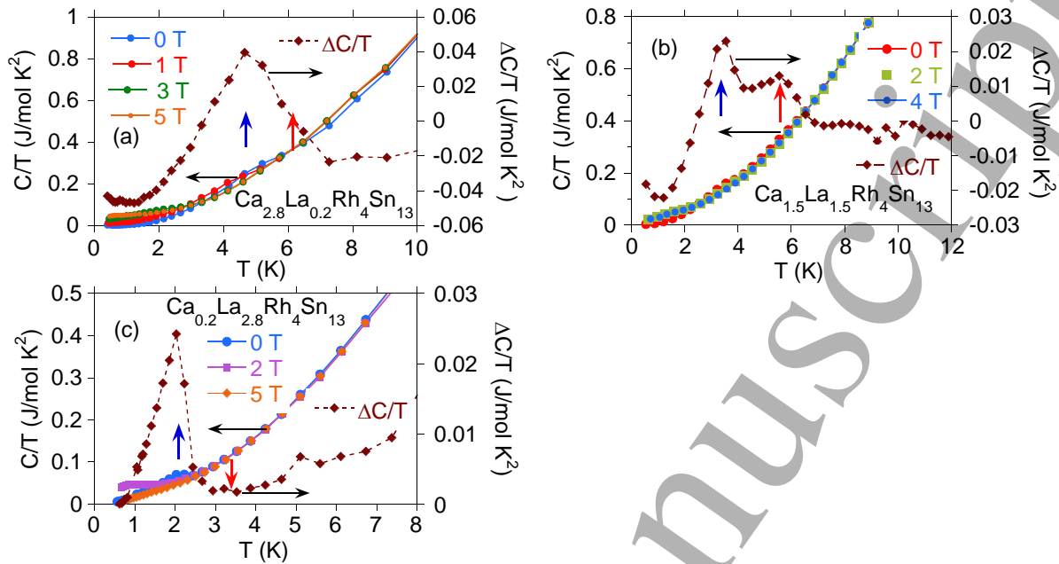
Figure 10. Temperature dependence of specific heat, C(T)/T and \Delta C(T)/T , for \text{Ca}_{3-x}\text{La}_x\text{Rh}_4\text{Sn}_{13} in various magnetic fields. \Delta C(T)/T is a difference of the C(T)/T data obtained at the zero magnetic field and the field B = 5 T. For \text{Ca}_{2.8}\text{La}_{0.2}\text{Rh}_4\text{Sn}_{13} (a), \Delta C(T)/T has only one broad maximum, well approximated by the function f(\tilde{\Delta}) , while the components x \geq 0.6 clearly show in the \Delta C(T)/T data two maxima due to presence of T_c^* and T_c superconducting phases [in panel (b) and (c)]. In all panels the vertical red and blue arrows indicate T_c^* and T_c , respectively.
