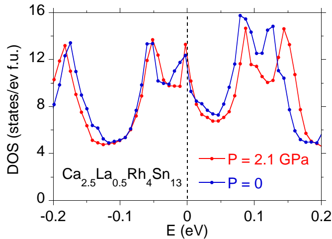
Figure A2. The total DOS near the Fermi energy calculated for \text{Ca}_{2.5}\text{La}_{0.5}\text{Rh}_4\text{Sn}_{13} at the pressure 0 and 2.1 GPa.
