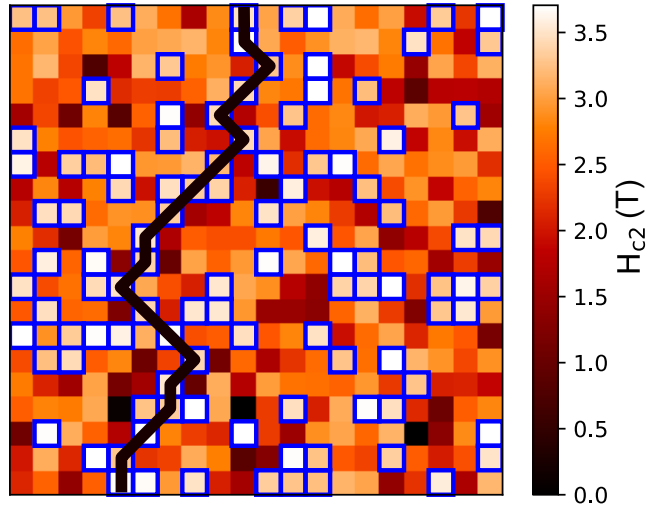
Figure 6. An example of the spatial distribution of local H_{c2} 's for a given realisation of the doping inhomogeneity. The local H_{c2} in squares framed with blue line is higher than the external magnetic field. They form a superconducting path across the entire system, marked by thick black line, so the magnetic field is smaller or equal to the global H_{c2}(T) .
