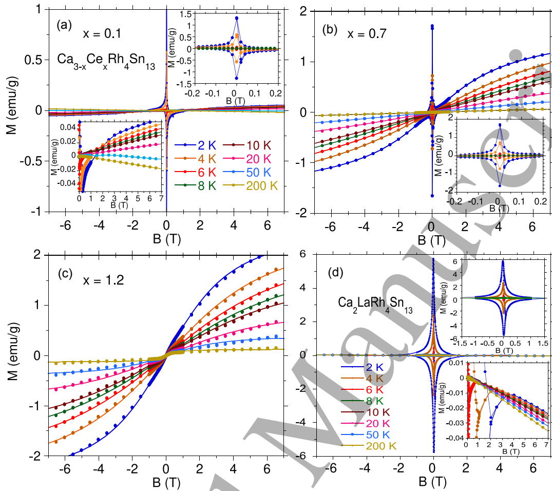
Figure 9. (a)–(c) Magnetisation M vs magnetic field B for \text{Ca}_{3-x}\text{Ce}_x\text{Rh}_4\text{Sn}_{13} at different temperatures. The insets exhibit hysteresis loops for superconducting state observed for the components x < 1.2 . A broad hysteresis loop suggests strongly inhomogeneous material. For x \geq 0.4 the solid lines are fits of the Langevin function to the magnetisation. (d) Magnetisation M vs magnetic field B isotherms for \text{Ca}_2\text{LaRh}_4\text{Sn}_{13} at different temperatures. Similar M vs B isotherms are observed for remaining \text{Ca}_{3-x}\text{La}_x\text{Rh}_4\text{Sn}_{13} compounds. The insets exhibit hysteresis loops for superconducting state and the diamagnetic M(B) behaviour, respectively. A broad hysteresis loop suggests strongly inhomogeneous material.
