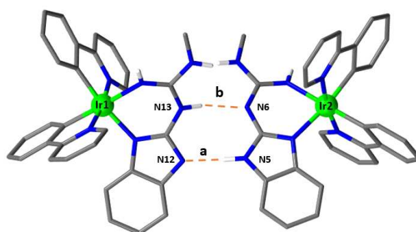
Figure 2. X-ray crystal structure of complex 1 with annotated NH...N contacts (orange); a) N5 \cdots N12 = 2.76 Å, NH \cdots N = 158°; b) N6 \cdots N12 = 2.91 Å, NH \cdots N = 161°. All CH-hydrogens and butyl chain are omitted for clarity.
