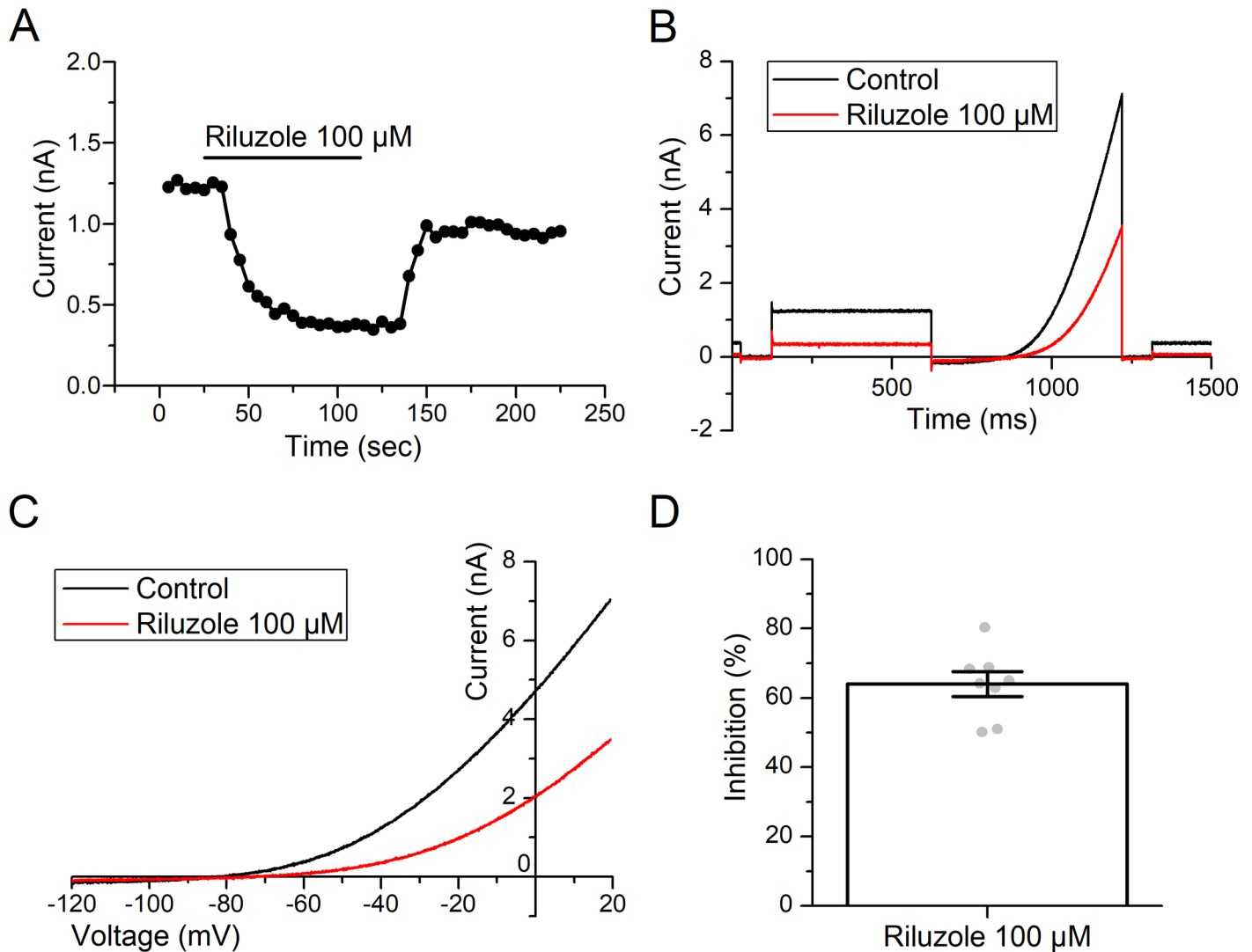
Fig 4. Riluzole (100 \mu M) is a potent inhibitor of human TRESK channels. (A) Bath application of riluzole (100 \mu M, black bar) rapidly and reversibly inhibited TRESK current measured at -40 mV. (B) Representative traces of TRESK currents in a single cell evoked using the “step ramp” protocol described in the methods in the absence (black) and presence (red) of riluzole (100 \mu M). (C) Representative current-voltage relationships for TRESK channels in a single cell in the absence (black) and presence (red) of riluzole (100 \mu M). (D) Inhibition of TRESK channel current at -40 mV by riluzole (100 \mu M) in 8 individual cells from 3 different recording days (gray dots). Error bars represent the mean \pm SEM.
