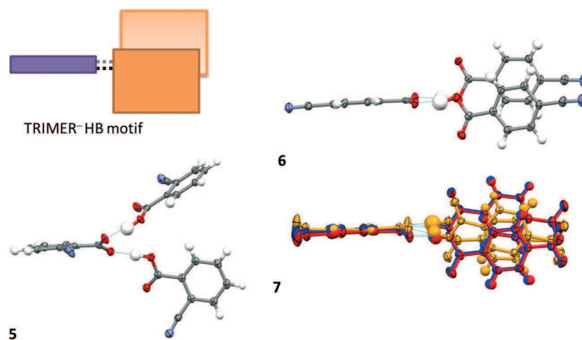
Fig. 2 The aggregation of \text{ACID}^- and \text{ACID} co-formers into \text{TRIMER}^- hydrogen bonded motifs via two \text{O}-\text{H}\cdots\text{O}^- CAHBs in complexes 5-7 (the three symmetry independent \text{TRIMERS}^- are overlaid for 7).
