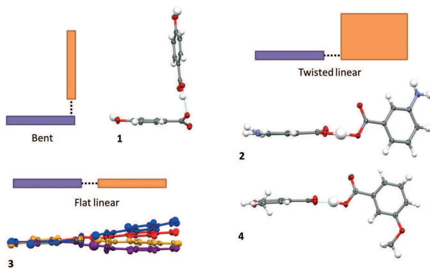
Fig. 1 The aggregation of \text{ACID}^- and \text{ACID} co-formers into \text{DIMER}^- HB motifs via a single \text{O}-\text{H}\cdots\text{O}^- CAHB with configurations bent (1), twisted linear (2 and 4) or flat linear (3: the three symmetry independent \text{DIMERS}^- are overlaid).
