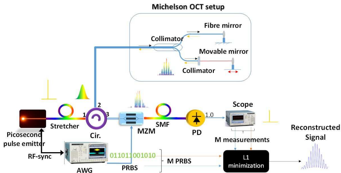
Figure 1. Schematic diagram of the proposed compressive sensing PTS-OCT system. AWG: arbitrary waveform generator, PRBS: pseudo random bit sequence, Cir.: Circulator, MZM: Mach-Zehnder modulator, SMF: Single mode fibre, PD: Photodetector.
