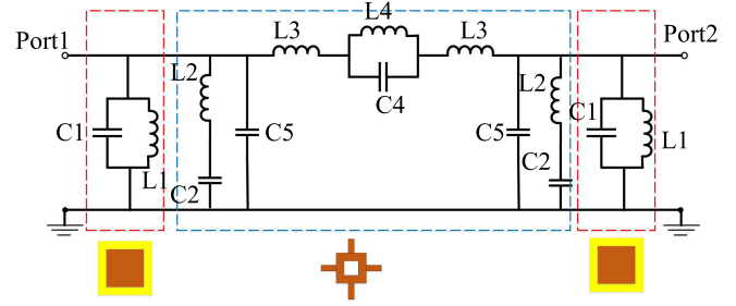
Fig. 2. Equivalent circuit model of the trilayer FSS working as a wideband passband filter.
