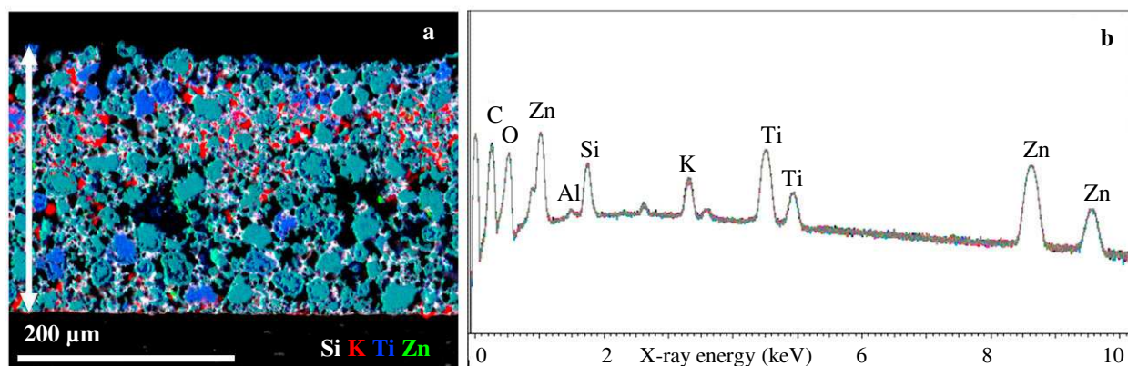
Fig. 1. SEM-EDX of section through WFPC2 paint: a) maps; b) 10 spectra, note that Mg and Fe are not seen.
