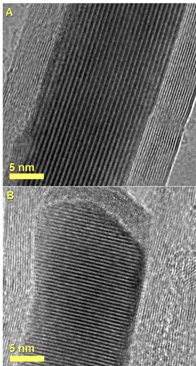
Figure 1. HRTEM micrographs showing the single-crystalline arrangement of the Fe 3 C crystals encapsulated inside the CNTs. Note the preferred 010 orientation of the Fe 3 C crystal in A and the preferred 100 orientation in B.
