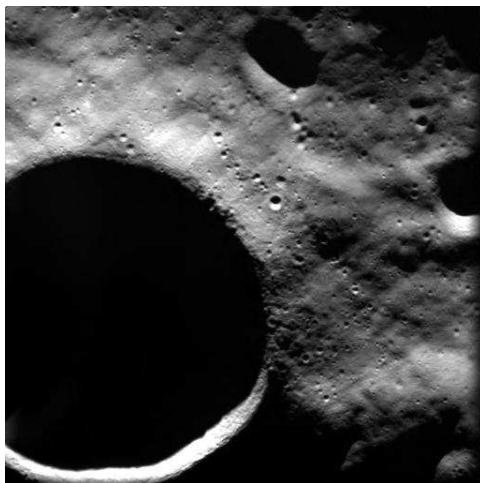
View of Shackleton Crater at the lunar South Pole taken by SMART-1. It is one of the deepest craters on the Moon, and its interior receives almost no direct sunlight. Deposits of water ice from comets may line the floor of the crater. Credit: ESA.
