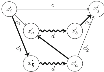
Fig. 6 Four ways to reduce the distance between x'_i and x'_j
