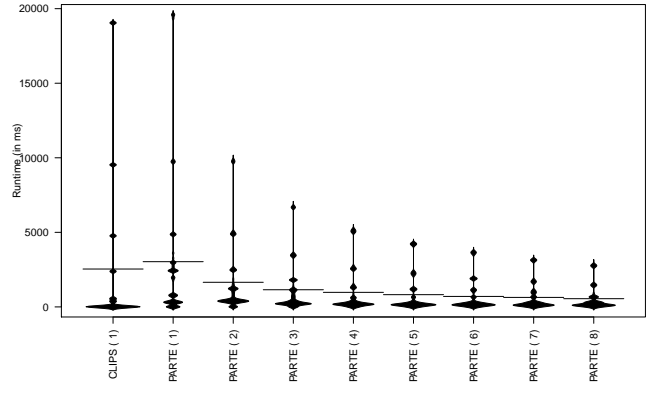
Figure 6. Beanplot showing distribution of benchmark results for 1 to 8 worker threads.
