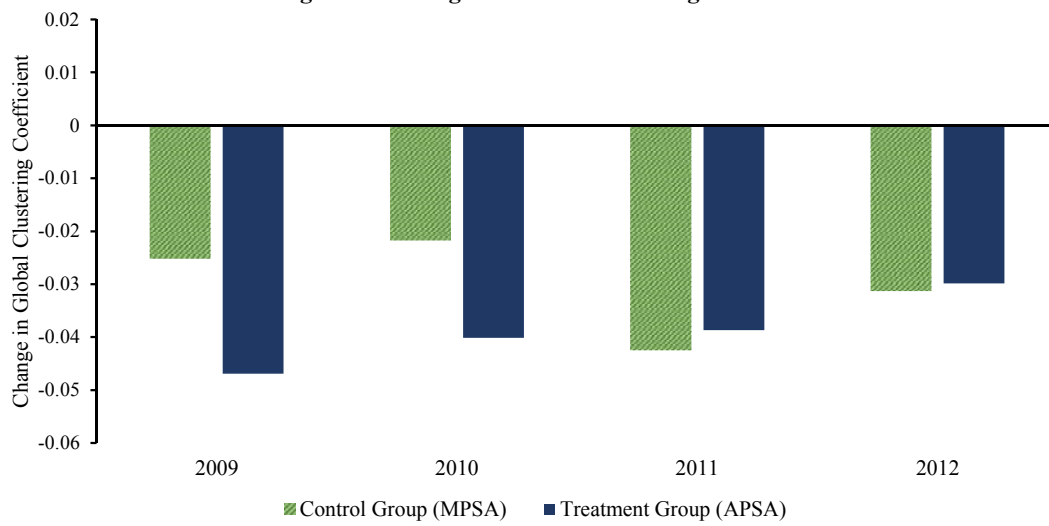
Figure 3 - Change in Global Clustering Coefficient
