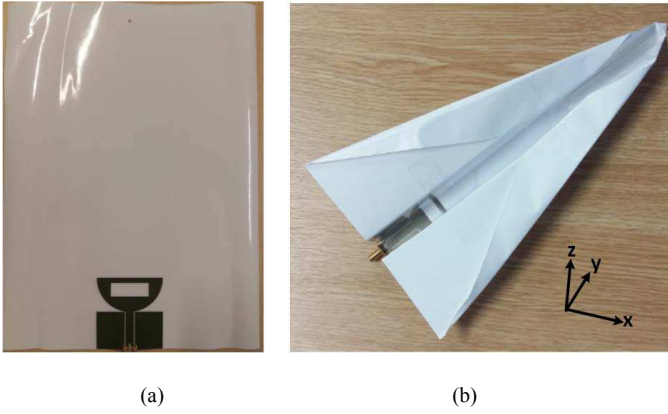
Fig. 5. Photographs of (a) the planar antenna on the extend paper substrate, and (b) the folded type 1 antenna
