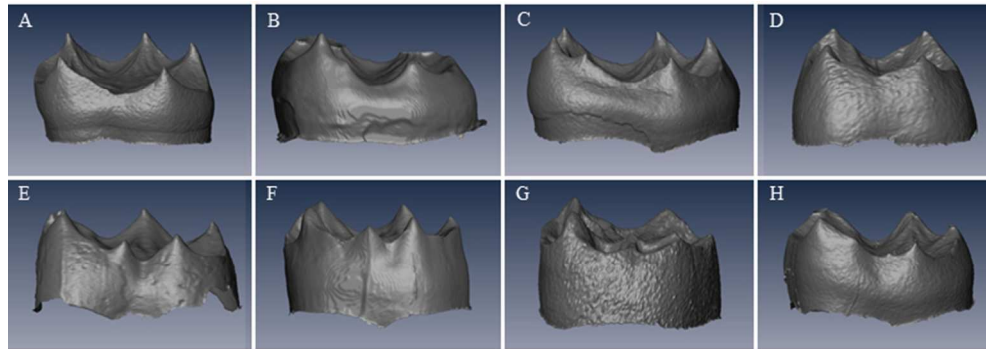
Figure 6. Types of LM C7 development (lingual view). A) LM C7 absent Skinner et al.'s (2008) type A (EDJ of P. troglodytes illustrated); B) Skinner et al.'s (2008) type B (EDJ of P. troglodytes illustrated); C) Skinner et al.'s (2008) type C (EDJ of P. troglodytes illustrated); D) Skinner et al.'s (2008) type D (EDJ of recent H. sapiens illustrated); E) Skinner et al.'s (2008) type E (EDJ of Homo sp. DNH 67 LRM1 illustrated); F) Skinner et al.'s (2008) type F (EDJ of H. neanderthalensis SD 780 LLM1 illustrated mirror-imaged); G) occlusal type (EDJ of H. neanderthalensis Vi 11-39 LRM3 illustrated); and entoconid type (EDJ of P. troglodytes illustrated). Mesial to the left.
