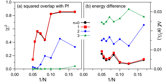
Fig. 2 (a) Squared overlaps |\chi|^2 of the exact Pfaffian state with the lowest L=0 Coulomb eigenstate at the half-filling of different LLs in graphene (at the same shift \sigma=3 ), plotted as a function of an inverse electron number N^{-1} . (b) Difference \Delta\mathcal{E} between the average Coulomb energy of the Pfaffian and the exact energy of the lowest L=0 Coulomb eigenstate, also at \nu=1/2 and \sigma=3 , and for different LLs of graphene, versus N^{-1} .
