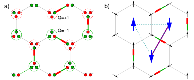
FIG. 1: (color online) a) Orientations of Ising spins on the links are mapped to a distribution of magnetic charges located at the extremities of each island. In kagomé-ice, the total charge at each vertex is constrained to |Q| = 1 . At low temperatures, vertex charges order such that all vertices of sublattice \alpha have charge Q_\alpha = (-1)^\alpha (as shown). To count the configurations corresponding to that NaCl charge-state, we map these to dimer coverings of the honeycomb lattice, where oriented dimers are present at all links connecting the minority charges of the adjacent vertices. b) To count the dimer coverings of the hexagonal lattice, we note that dimers present on the hexagonal lattice can be mapped to broken links of the antiferromagnet on the dual triangular lattice. The particular configuration shown contains the unit-cell of the groundstate, formed by the three highlighted plaquettes. Arrows shown at the vertices display the direction of the local dipole moment.
