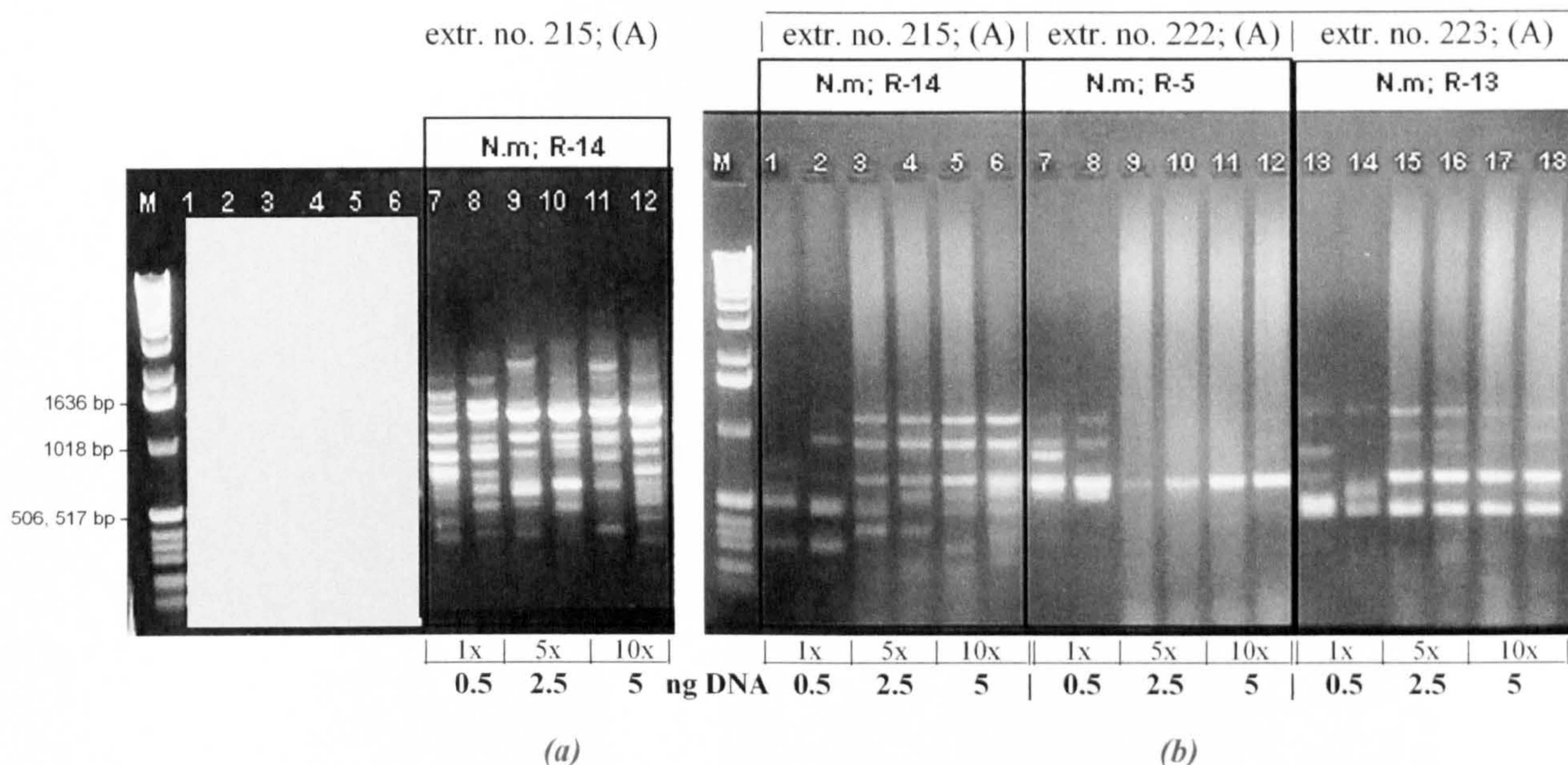
Figure 23 – RAPD-PCR experiments with formalin-arDNAs of N. micronychodon (N.m) (different arDNA extracts and from different fish individuals) using RAPD Primer 37.
