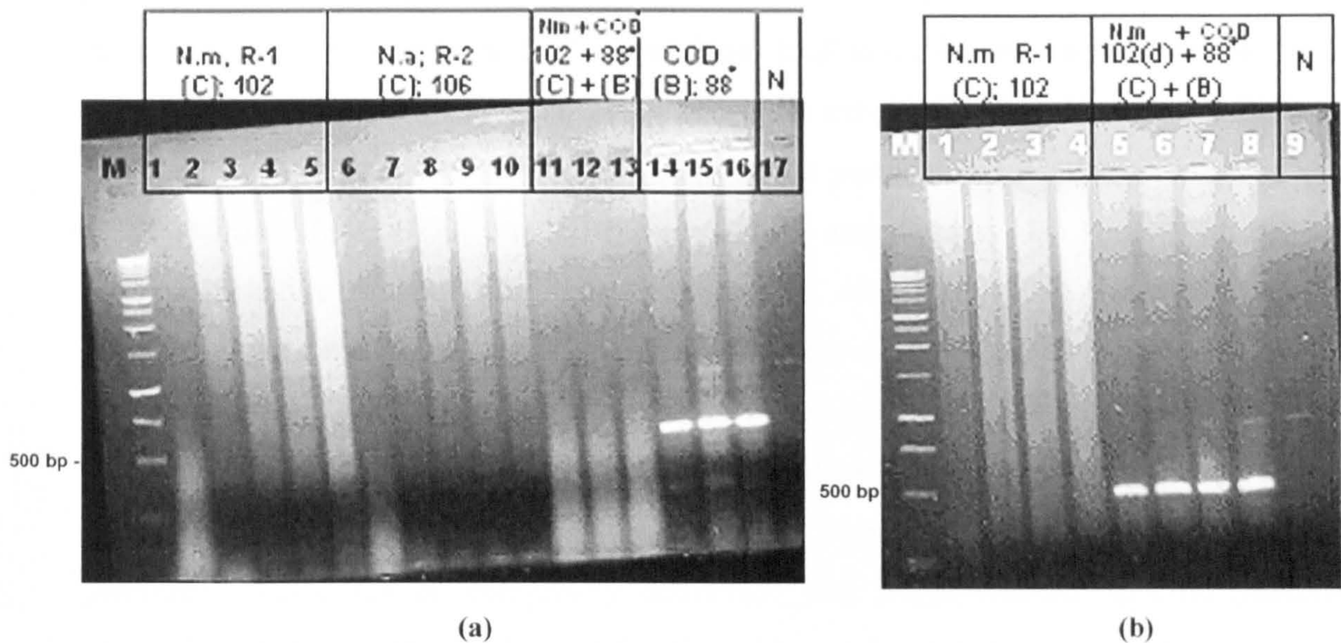
Fig. 11 – Strong PCR inhibition was proved by mixing control DNA of frozen cod (produced by protocol (B)) and formalin-arDNA of Nezumia produced by protocol (C). Mitochondrial PCR amplifications of the COIII gene were tested.
