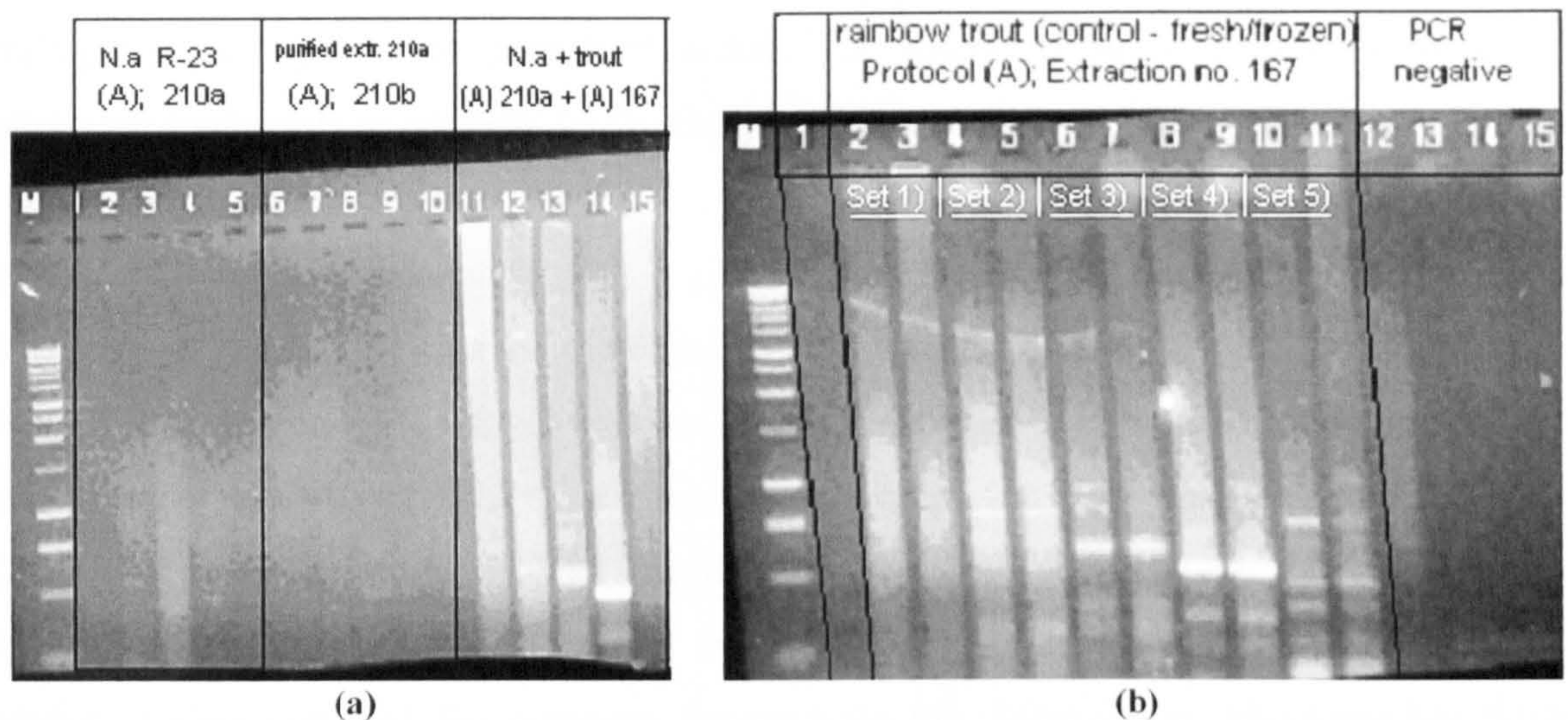
Fig. 14 – Inability to amplify the regions of mitochondrial DNA in arDNA extracts produced by protocol (A) (Lanes: 1-10 on gel (a)) were not caused by “diffusible” PCR inhibitors. This was demonstrated by mixing control DNA of fresh/frozen rainbow trout and arDNA of formalin-fixed Nezumia aequalis (gel (a)-Lanes: 11-15). The same mitochondrial regions were PCR amplified in mixed DNA extracts (arDNA of Nezumia + DNA of rainbow trout) (Lanes: 11-15 on gel (a)) and in DNA extract of trout alone in duplicate PCR amplifications (Lanes: 2-11 on gel (b)) “M” indicates size marker fragments - 1Kb DNA Ladder (Promega). N.a – Nezumia aequalis R - the identifier of the fish individuals (R-23 is fish individual no. 23) (A) – DNA extracts produced by protocol (A).
