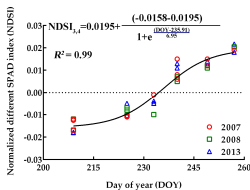
Figure 6. Critical NDSI_{L3,4} data points used to define the changes in the NDSI_{L3,4} curve when data of high-yield targets were pooled. The solid line is the critical NDSI_{L3,4} change curve ( NDSI_{3,4} = 0.0195 + \frac{-0.0158 - 0.0195}{1 + e^{\frac{DOY - 235.91}{6.95}}} ; the A_1 , A_2 , x_0 , and dx values differ in terms of their effect on NDSI_{L3,4} trends) of high-yield target rice in the Yangtze river valley.
