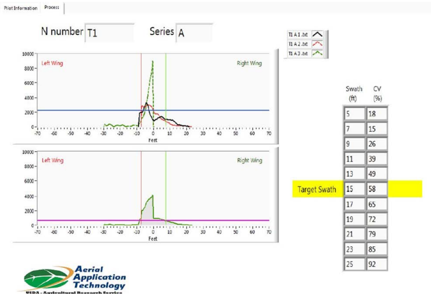
Figure 2. Sample average “bad” pattern from the V6A at 4 m height and 1 m/s. Due to the height, a smaller droplet spectra and crosswind from the left, many of the droplets were not able to land on the target string and thus, resulted in a “poor” pattern and large CV.
