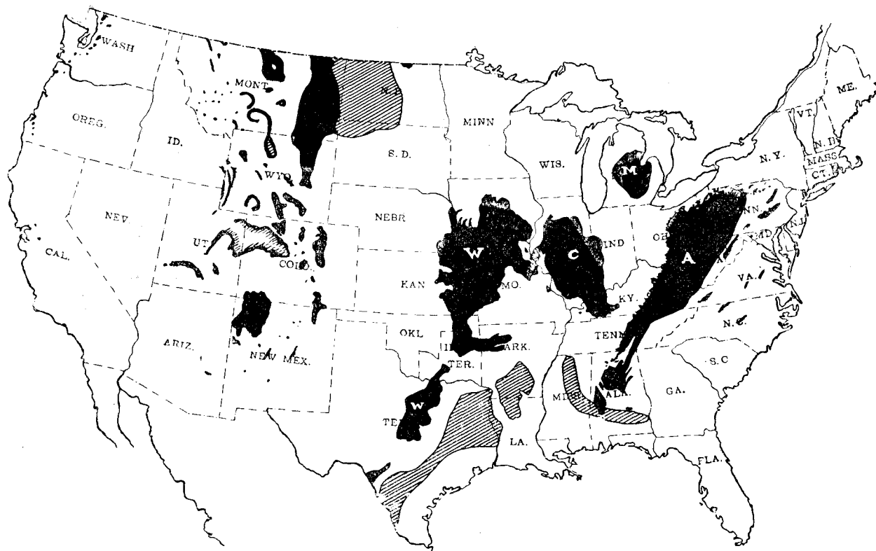
Fig. 13. A coal map of the United States. The coal east of Nebraska is of Carboniferous age; west of Nebraska the coal is of Cretaceous age. A, Appalachian coal field; C, Central coal field; W, Western coal field; M, Michigan coal field; Rhode Island coal field. Ruled area, lignite. Modified after maps of U. S. G. S.
