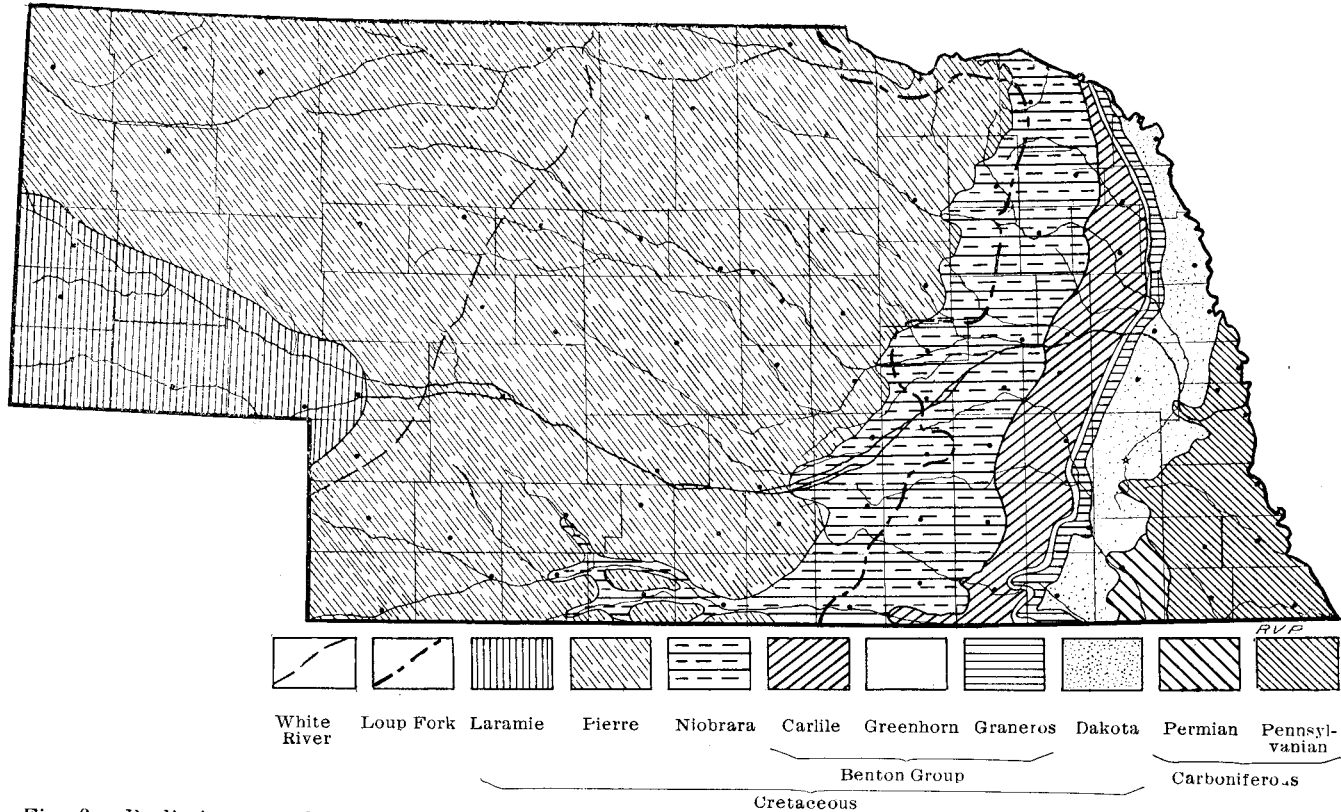
Fig. 2. Preliminary geological map of Nebraska, showing distribution of Pre-tertiary formations. The eastern limits of the Loup Fork and White River respectively, are indicated by dotted lines.
