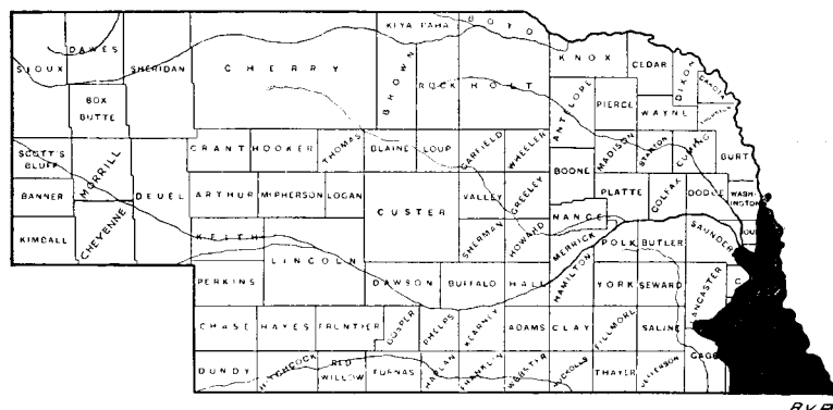
Fig. 3. Exposure of the Pennsylvanian in Nebraska. In the eastern edge of this area the coal bed varies from one foot in thickness to approximately three feet. In the western edge it pinches out to a few inches.
