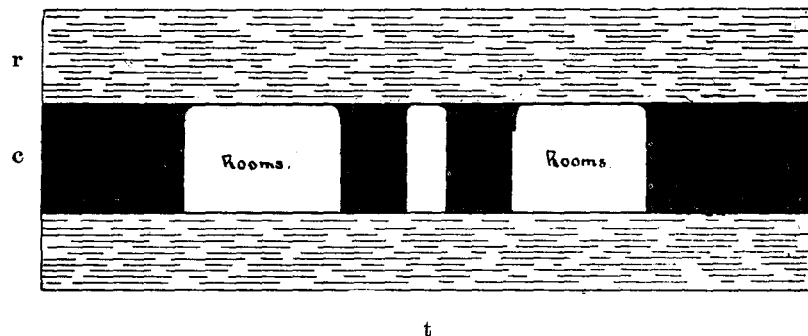
Fig. 8. Sectional view at Honey Creek Coal Mine, tunnel No. 2, showing room and pillar method of mining. t, tunnel No. 2; r, roofing shale; c, coal bed with a maximum thickness of 35 to 36 inches, a minimum of 29 1/4 inches and an average of 32.9, or 33 inches in round numbers.
