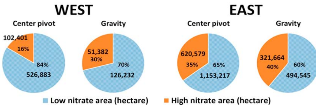
Fig. 9. Areas of high (or at the maximum contaminant level, MCL) nitrate concentrations ( \geq exceeding 10 mg NO_3 -N/L) and low (below the MCL) nitrate concentrations ( < 10 mg NO_3 -N/L) under different irrigation systems in western and eastern Nebraska.
