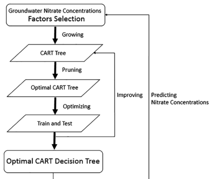
Fig. 2. The CART model for estimating groundwater nitrate concentrations.
