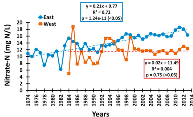
Fig. 5. Long-term trends of groundwater nitrate concentration (1974–2013) in western and eastern Nebraska.
