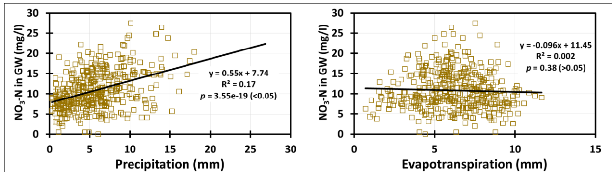
Figure S3. Correlation of precipitation and evapotranspiration with nitrate concentration in groundwater.
