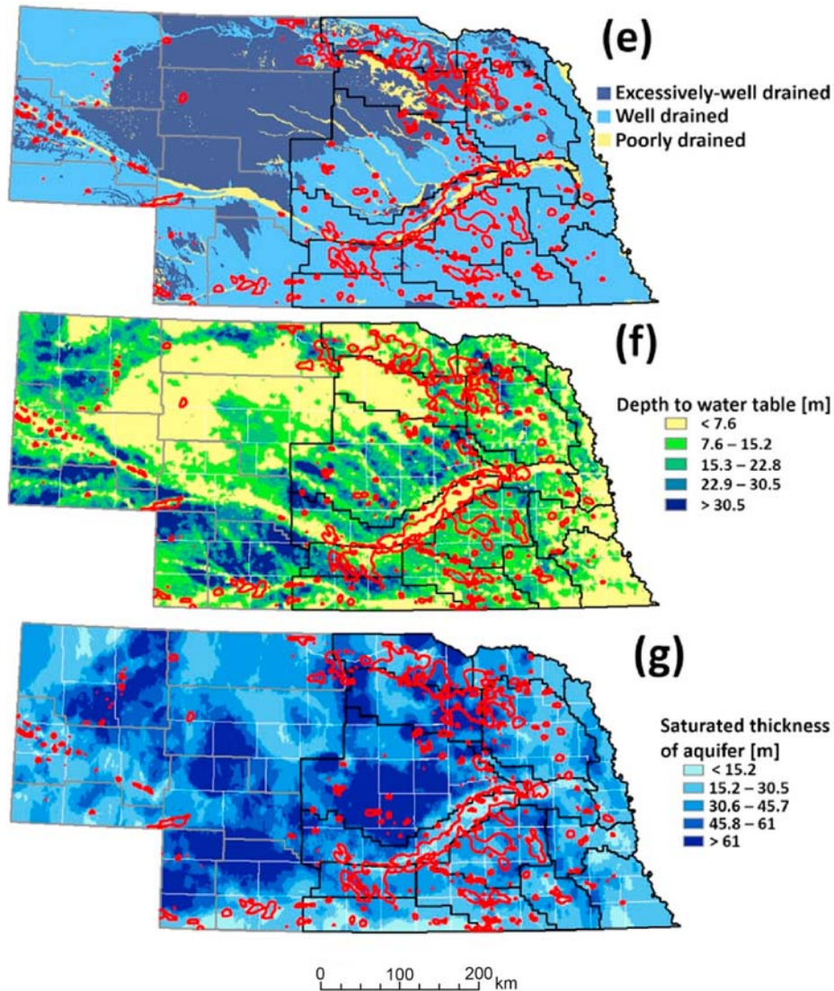
Fig. 7. (continued) The original map is of sufficient resolution (30 m) to show individual fields planted to corn or soybeans. Natural factors: (e) Soil drainage capacities, (f) depth to water table, and (g) saturated thickness with groundwater nitrate concentrations within the red outlined areas of \geq 10 mg \text{NO}_3\text{-N/L} during 2004–2013.
