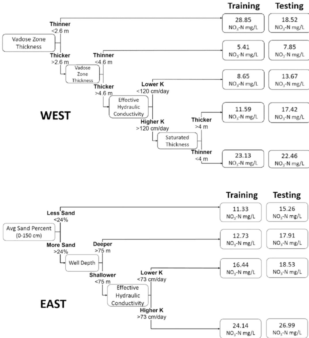
Fig. 11. The output of CART pruning tree for groundwater nitrate concentration prediction in western and eastern Nebraska.
