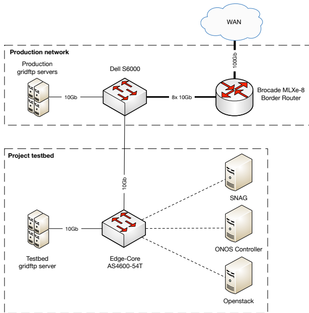
Figure 5: Network Topology
