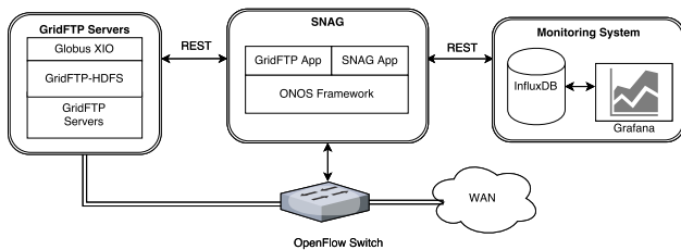
Figure 4: SNAG Components [4]
