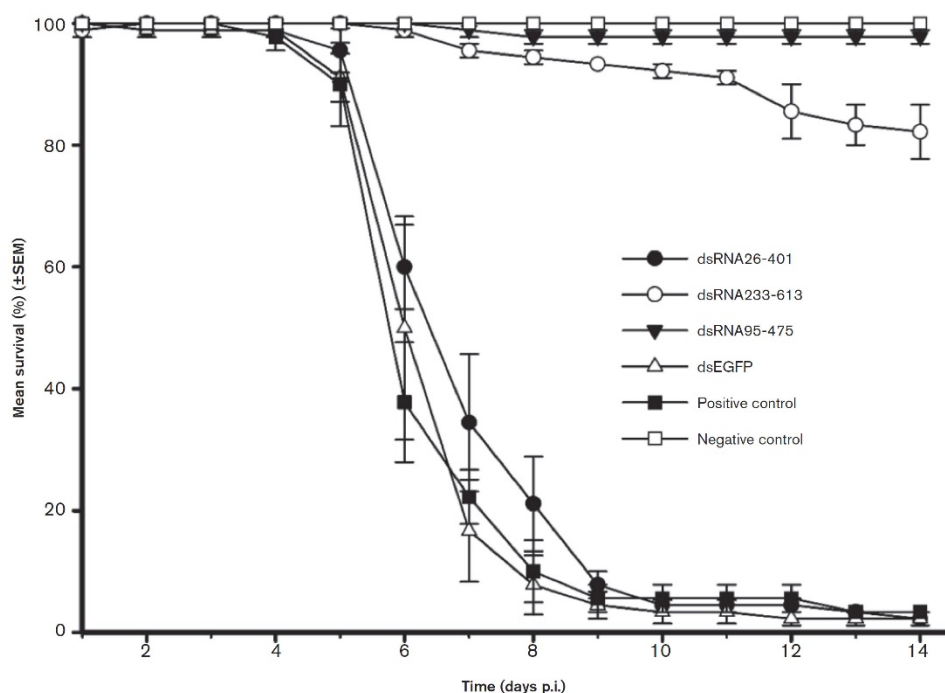
Figure 4. Shrimp survival post-administration with novel dsRNAs (dsRNA26-401 and dsRNA233-613) compared with previously reported dsRNA (dsRNA95-475) and heterologous dsRNA (dsEGFP) post 48 h IMNV infection. Data represent mean \pm SEM; n = 90 animals per treatment except for the negative control group, n = 30 animals.
