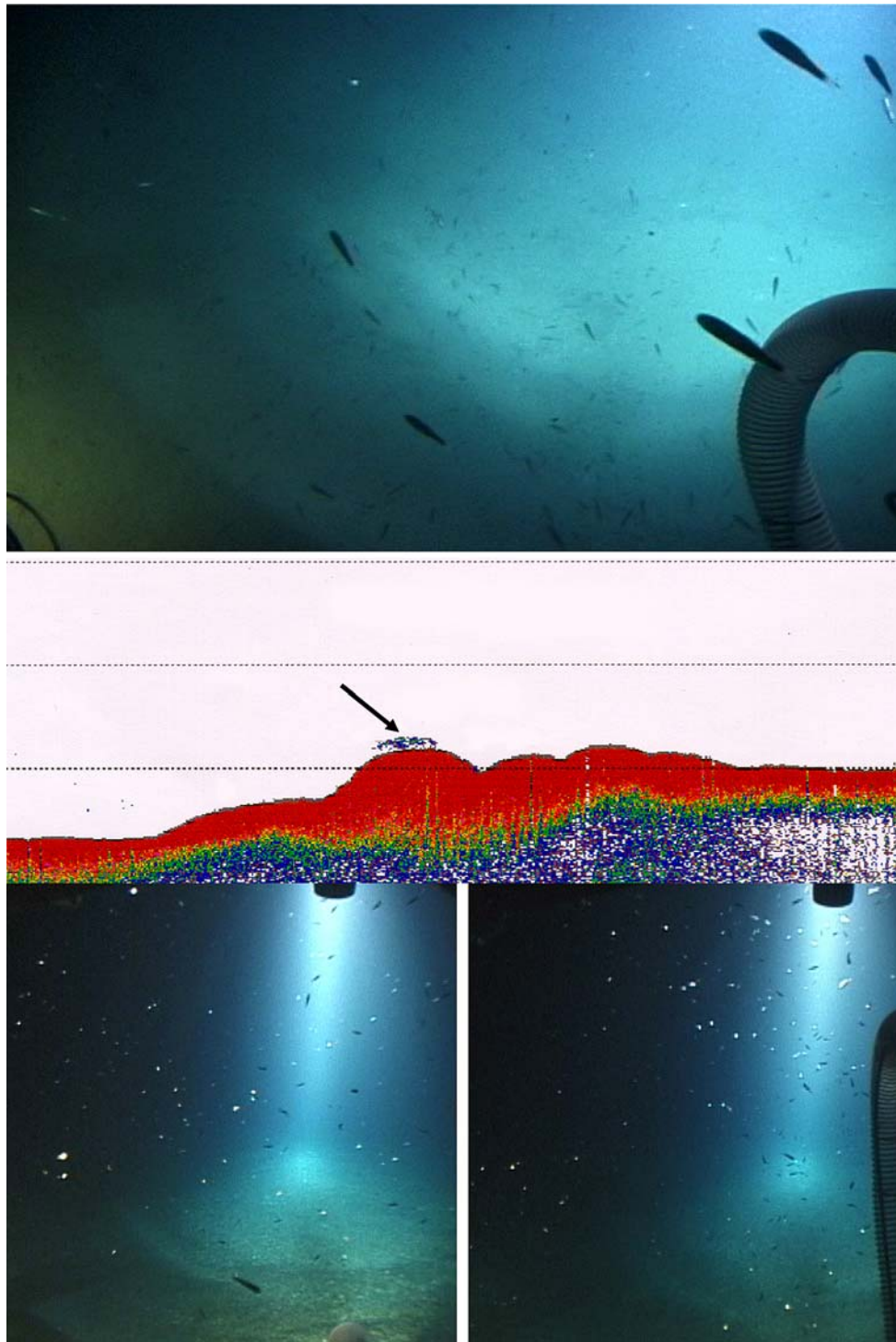
Fig. 3 Dense near bottom aggregations of mesopelagic fishes. Top panel is mostly Ceratoscopelus maderensis from JSL dive 4204 (27 July 2000, 0942 hours) over muddy substrate at 596 m at the HMS study area. Center panel is an echosounder profile of a coral bank in the LMS area taken just before JSL dive 4363, illustrating a large swarm of mesopelagic animals near bottom at top of ridge ( arrow ).
