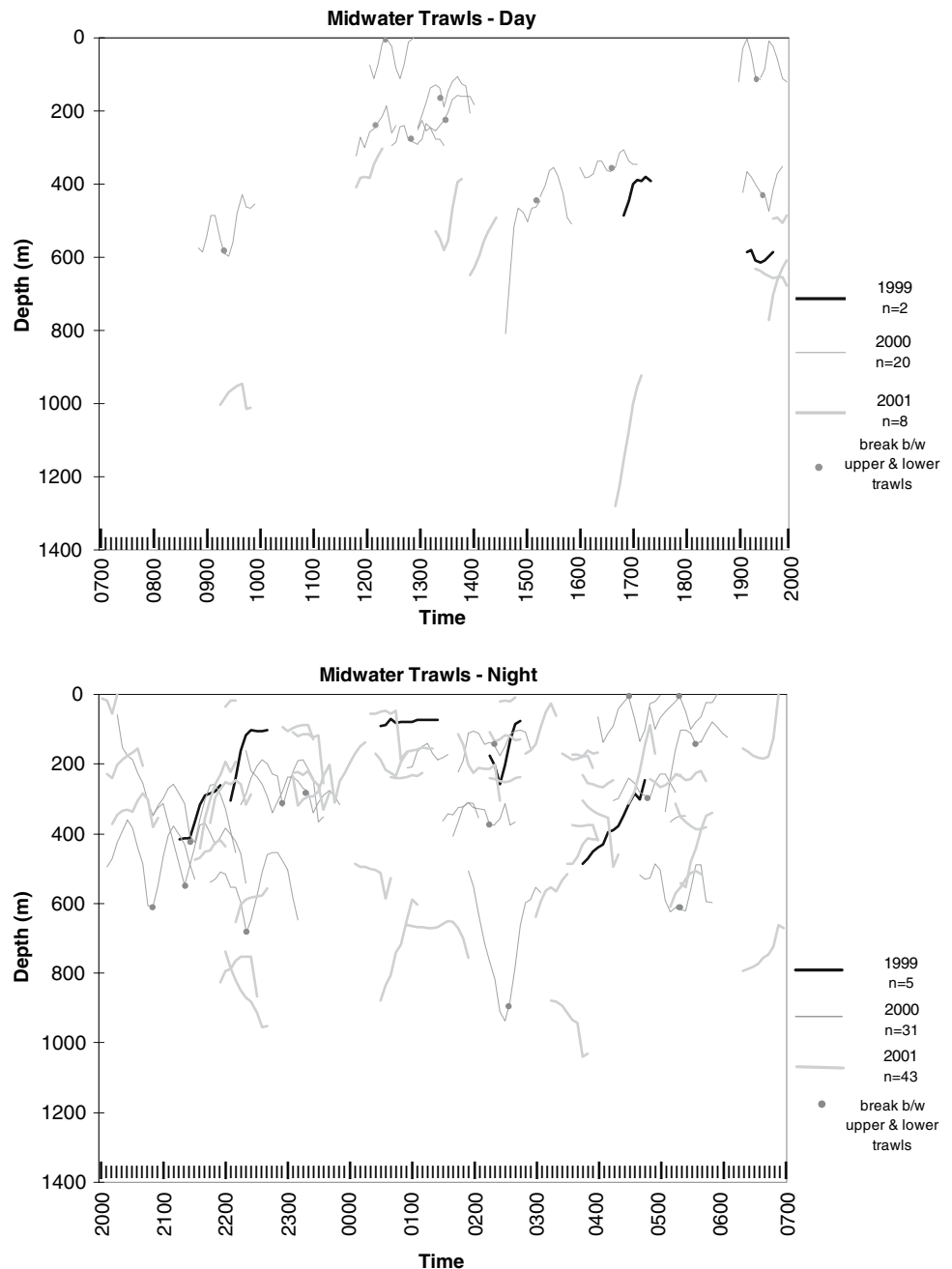
Fig. 2 Depth-time profiles for Tucker Trawl samples from 1999 through 2001 cruises. a Daytime samples. b Nighttime samples. Four nighttime samples are overlapped by others and thus appear to be missing in figure
