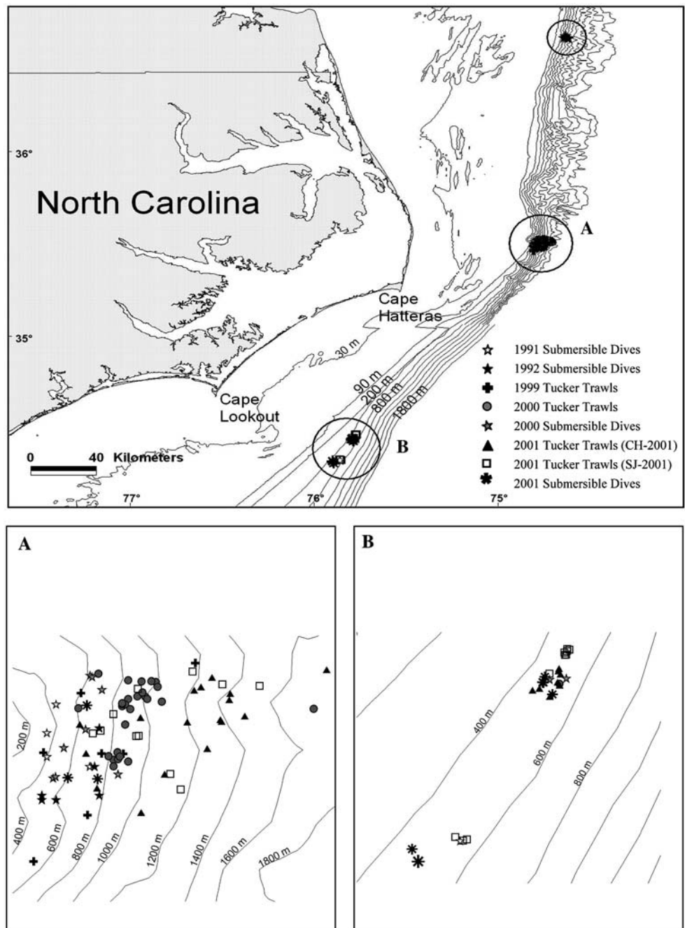
Fig. 1 Station map for Tucker trawls and submersible dives from three general areas along the Virginia and North Carolina continental slope. Upper Circle Virginia Middle Slope stations (VMS in text); Circle and Inset A Hatteras Middle Slope (HMS in text); Circle and Inset B Cape Lookout Middle Slope (LMS in text). Inset for VMS not provided because of the very close proximity of stations and small sample size (four dives)
