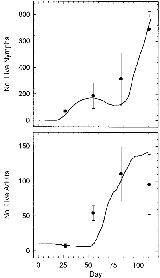
Fig. 5. Observed (circles, mean and 95% confidence intervals) and simulated (solid line) population development of L. campestris in the first validation test conducted from 26 May to 15 September in a screened shed in Madison, WI.
