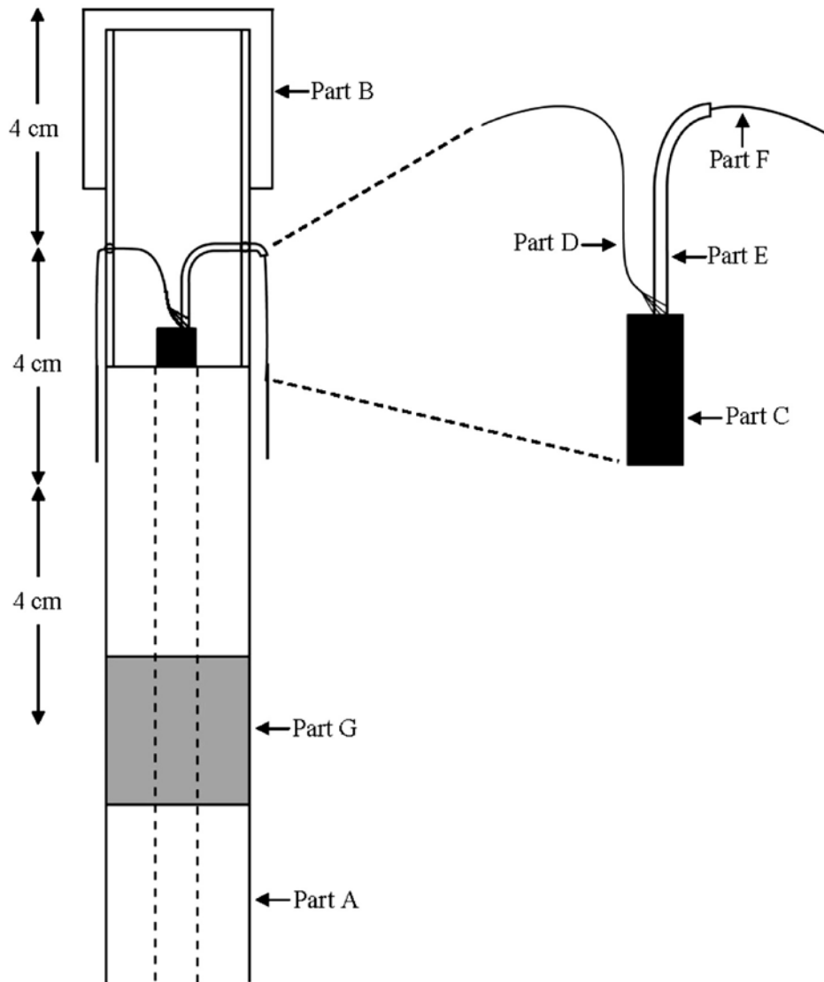
Figure 1. Underwater telemetry antenna schematic for locating submerged radiocollars. Items needed to complete antenna assembly were: schedule-40 polyvinyl chloride (PVC) pipe (Part A), PVC cap (Part B), and RG-58 coaxial cable (Part C). The mesh wires located inside of the coaxial cable were twisted into a single 7.5-cm wire conductor (Part D). We removed 3 cm of insulation (Part E) to expose the single center conductor (Part F). To reduce buoyancy, an optional plug (approx. 2.5 cm) made of room temperature vulcanizing (RTV) silicone sealant can be inserted approximately 12 cm from the antenna end (Part G). Figure developed by B. Washington, Mississippi State University.
