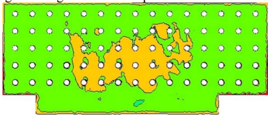
Fig.14. Cross-section temperature distribution at Z=1m.
