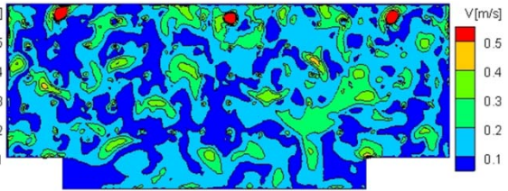
Fig.5. Cross-section velocity distribution at Z = 1.7 m.
