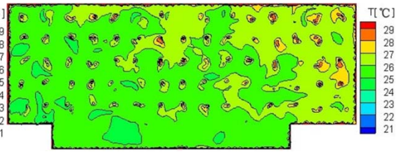
Fig.3. Cross-section temperature distribution at Z = 1.7 m.
