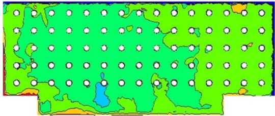
Fig.12. Cross-section temperature distribution at Z=0.7 m.
