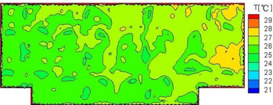
Fig.7. Cross-section temperature distribution at Z = 2.3 m.
