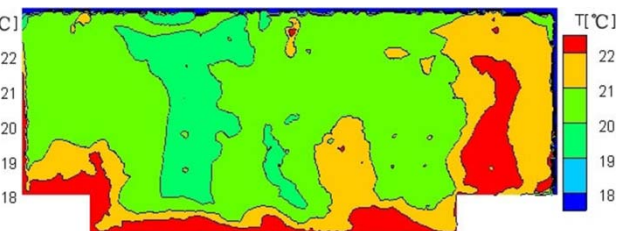
Fig.9. Cross-section temperature distribution at Z=1.7m.
