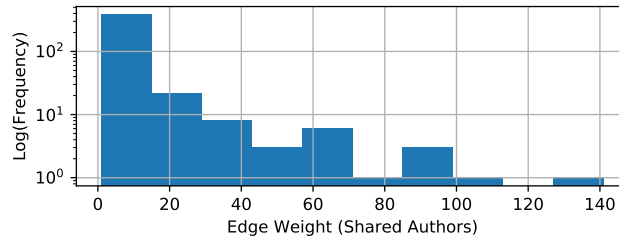
Fig. 2. Distribution of shared authors across domains, presented in log-scale.
