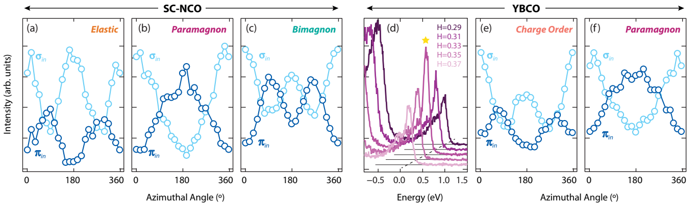
FIG. 5. (a)–(c) Azimuthal dependence of elastic scattering, paramagnon excitation, and bimagnon excitation in SC-NCO. (d) Low-energy excitations of YBCO around the charge order wave vector. (e) and (f) Azimuthal dependence of the charge order scattering and the paramagnon excitation in YBCO.
