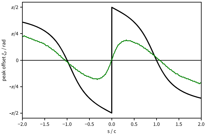
Figure 15. Analytic phase-curve offset for an analogous one-dimensional shallow-water model along the equator in the absence of rotation. The black line is Equation (23), and the green line shows the results of a numerical simulation that includes nonlinear terms, momentum drag, and a nonsmooth forcing similar in form to Equation (12).
