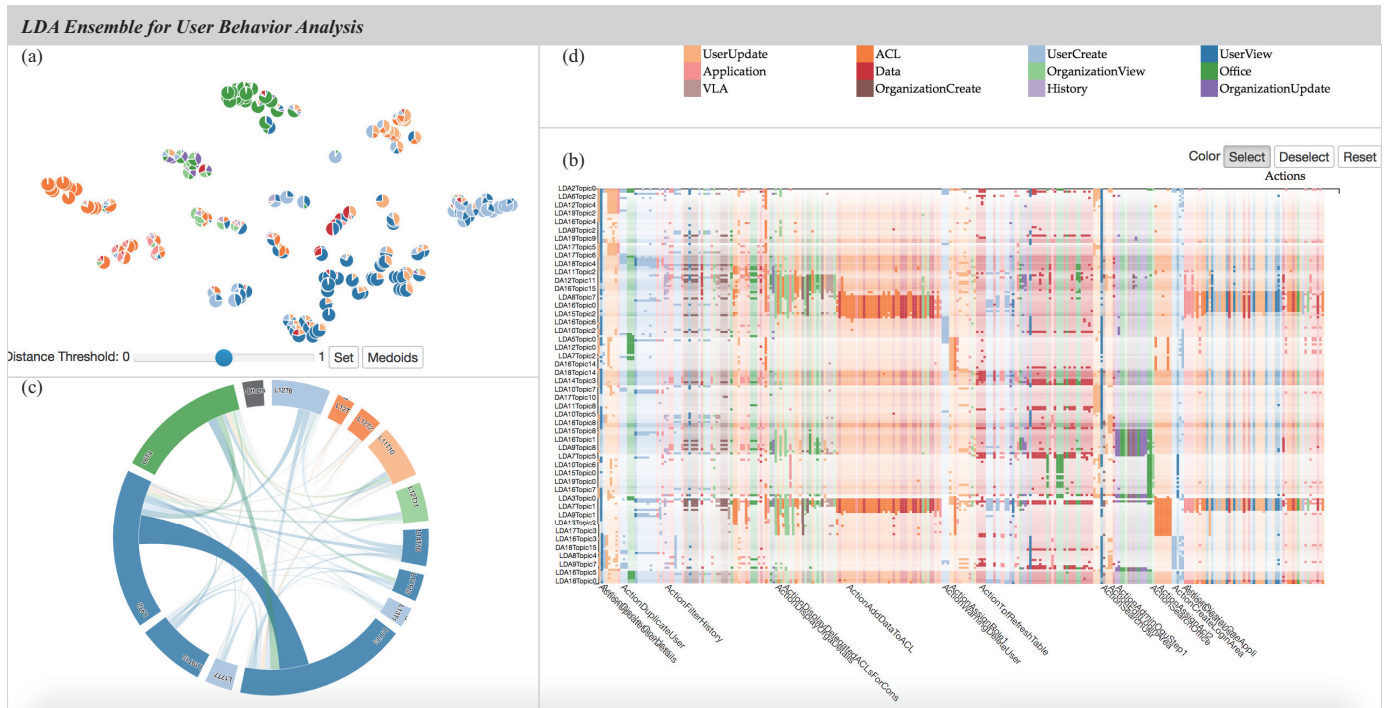
Fig. 1. Visual interface for exploring results of ensembles of topic models. The visualization system includes (a) topic projection view, (b) topic-action matrix, (c) topic chord diagram, and (d) color labels of action classes. We label the topics as “LDA i Topic j ” to reflect the LDA run and topic number.
