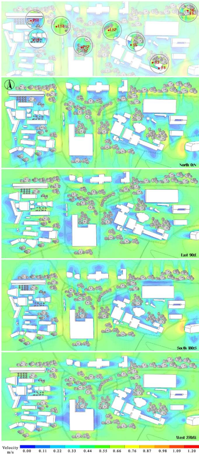
Fig. 13. Results of simulated wind velocity in UM campus from 4 directions (0:North, 90:East, 180:South, 270:West) with speed of 1.1 m/s (PS1-2: partially shaded 1-2, US1-2: unshaded 1-2, FS: fully shaded, S1-6: space 1-6).
