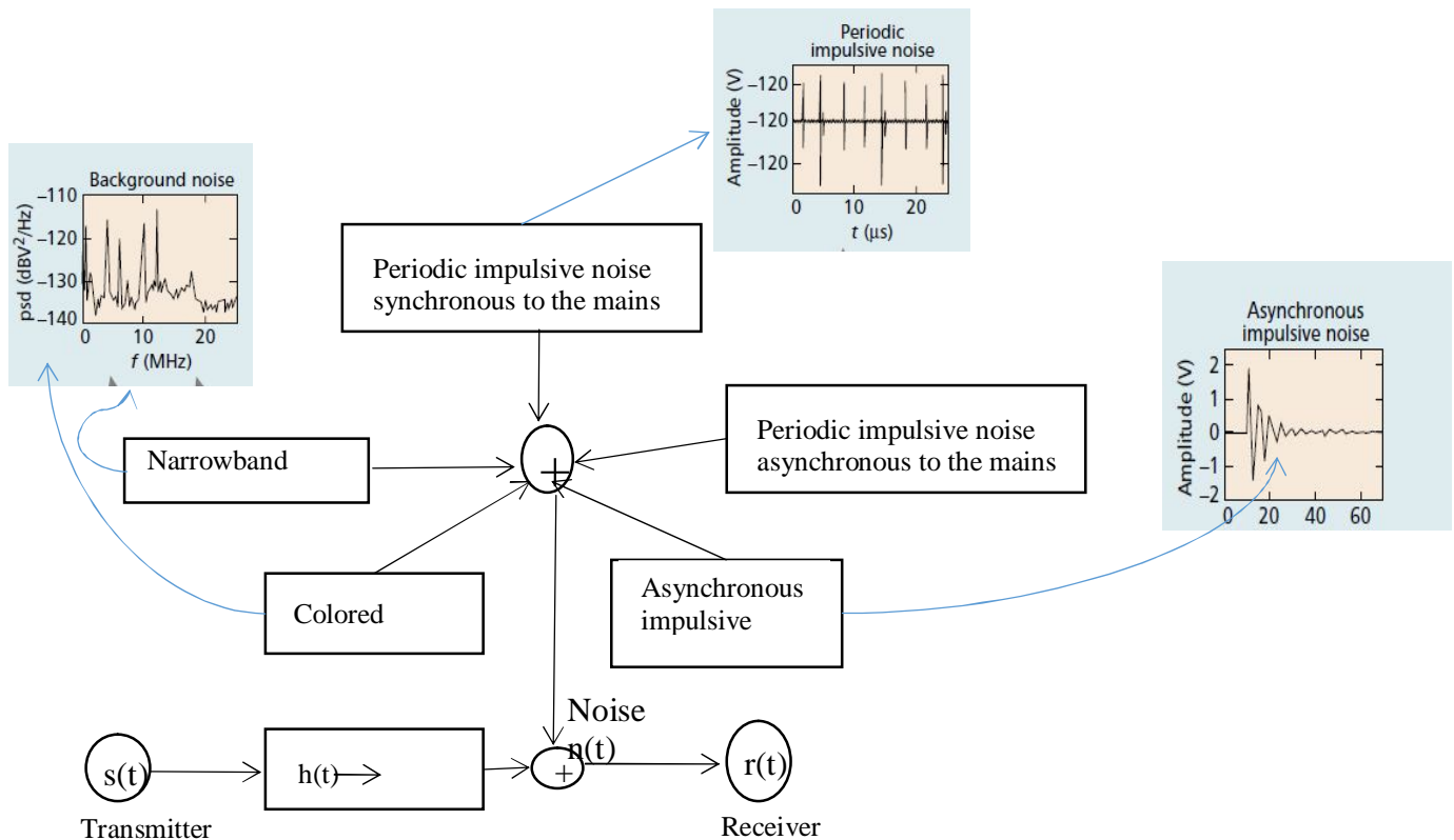
Figure 1 Noise Scenario in PLC
