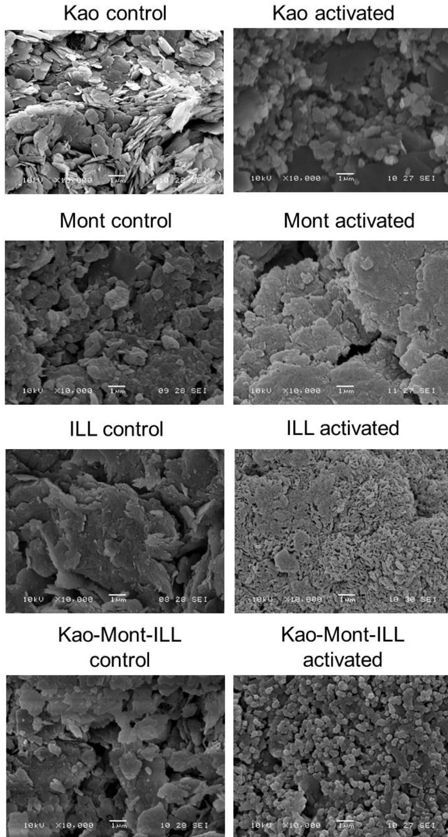
Figure 3: SEM images of control and activated samples of kaolinite, montmorillonite, illite and a mixture of all three.
