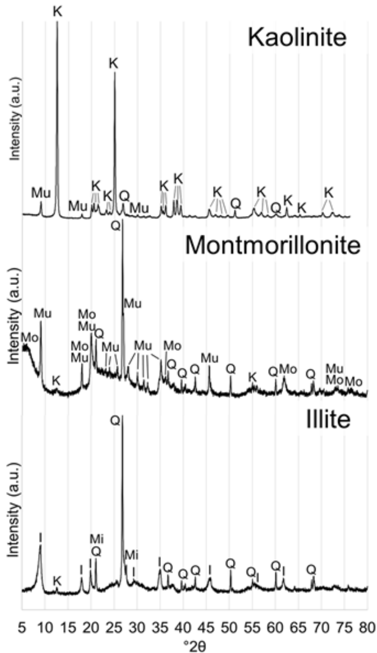
Figure 1: PXRD patterns of a) Kaolinite precursor; b) K10 montmorillonite precursor; c) IMt-2 illite precursor. Indexed as: I = illite; K = kaolinite; Mi = microcline; Mo = montmorillonite; Mu = muscovite; Q = quartz.
